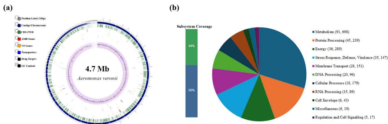
Fig. 3 Circular genomic map for A. veronii Fsp5. From the outside to the center are the assembled contigs, open reading frame (ORF), CDS in the forward strand, CDS with similarity to known antibiotic resistance genes, CDS with similarity to virulence factors, transporters, drug target, and GC content (a), subsystems information. Subsystem coverage showed that 44% of genes (2,055) were assigned to subsystems, while the remaining 56% (2,565 genes) were not classified within the subsystem categories (b).
