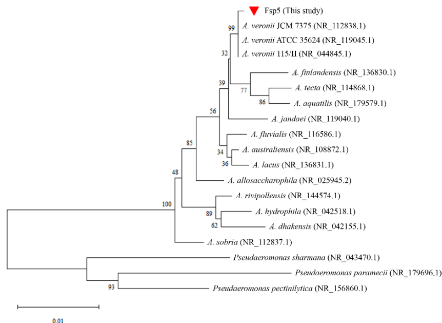
Fig. 2 Phylogenetic tree derived from 16S rRNA gene sequences. The tree was constructed using the Neighbor-Joining method. Percentage bootstrap values (1000 replicates) are shown at each branch point. The scale bar 0.01 represents substitutions per nucleotide position.
