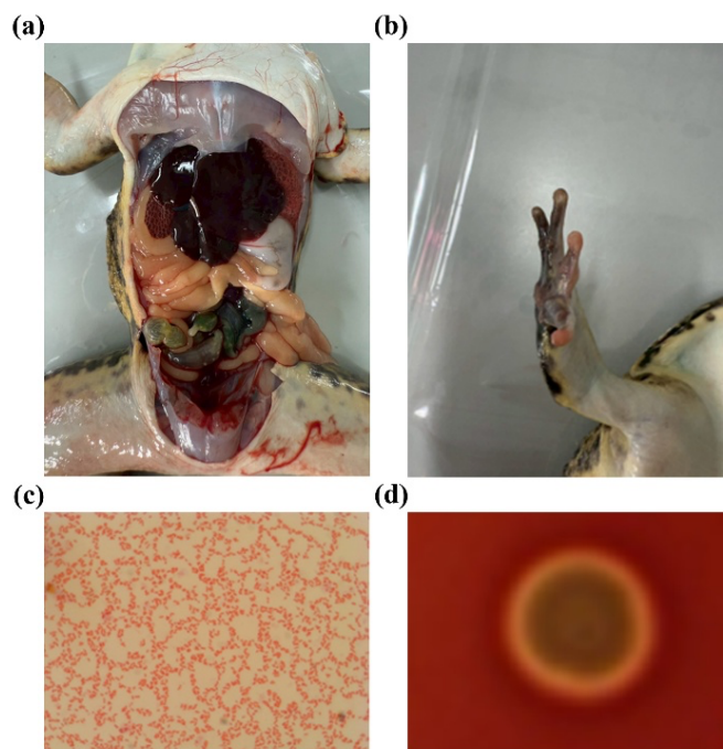
Fig. 1 Internal organs of diseased frogs (a), External lesions of diseased frogs (b), Gram staining of the bacterial isolate (c), \beta -hemolysis of erythrocytes on blood agar (d).
