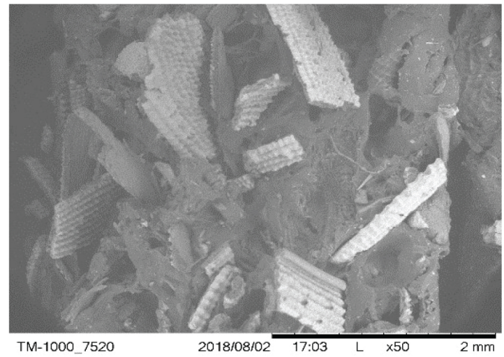
SEM micrographs of tensile fracture surfaces of RHs/NR composites
