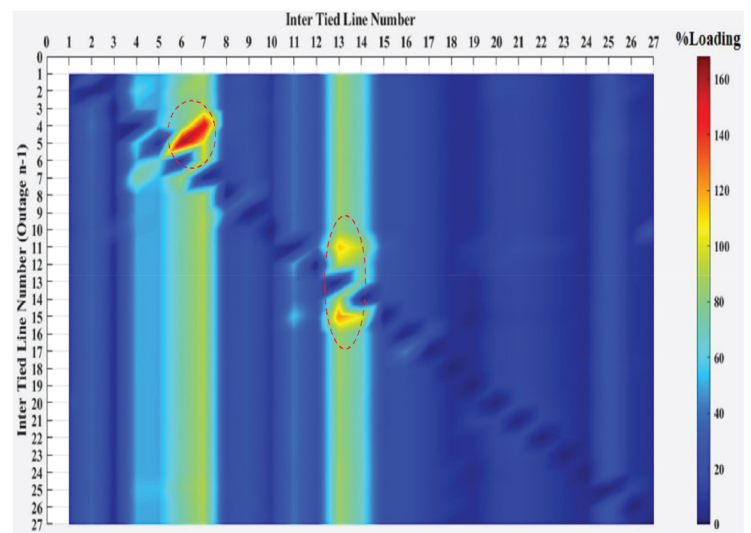
Inter-tied lines load percentage assessment in case of loss of each inter-tied line.
