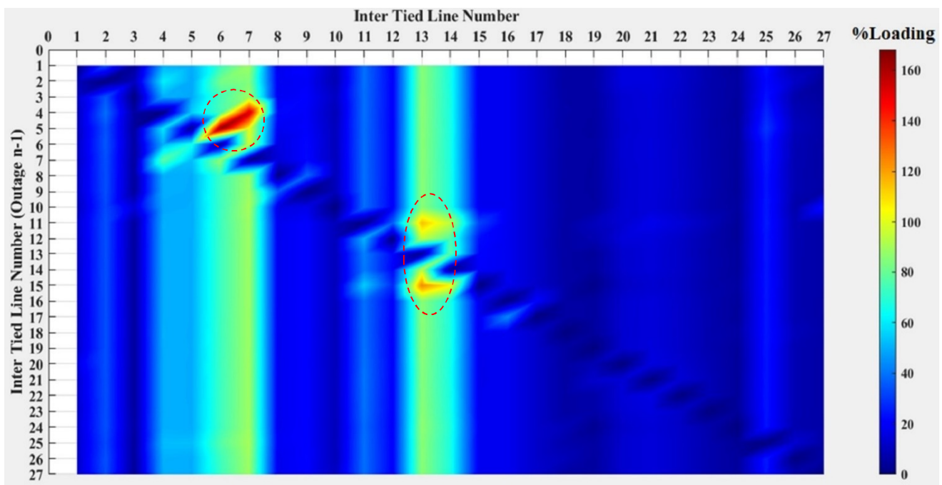
Fig. 3 Inter-tied lines' load percentage assessment in case of loss of each inter-tied line.
