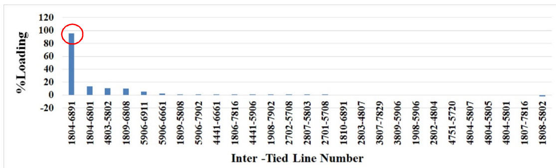
Fig. 4 Priority transmission line sequence in the case of the fifth line (1810 – 6891) is disconnected.
