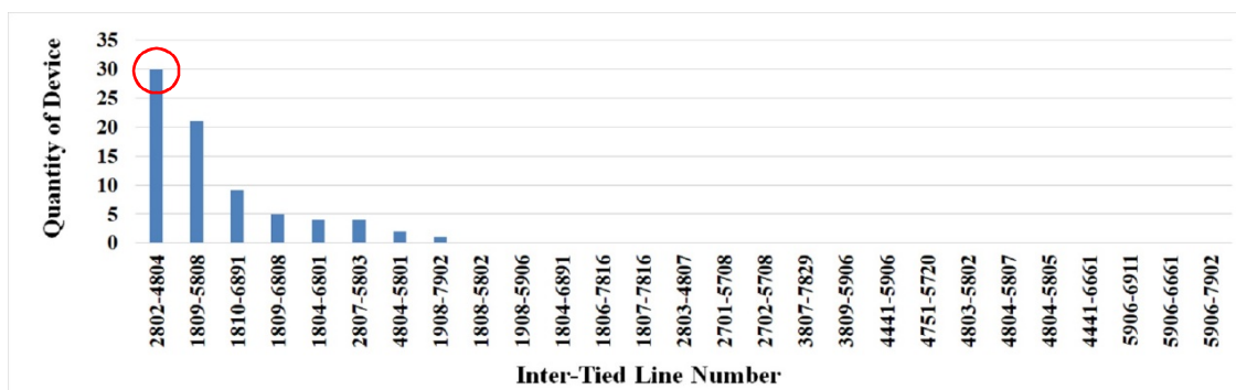
Fig. 5 The sequence of severity under the inter-tied lines that was disconnected.
