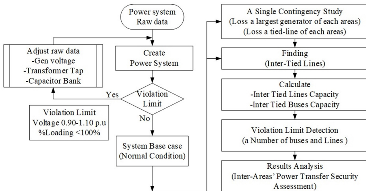
Fig.1 Procedure diagram for the assessment of inter-area power transfer capability.
