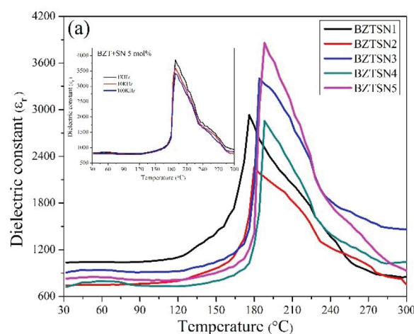
Dielectric Properties of (1-x)\text{Ba}(\text{Zr}_{0.2}\text{Ti}_{0.8})\text{O}_{3-x}\text{SbNb}_04 sintering at 1,150\text{ }^{\circ}\text{C}
