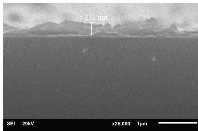
Cross-section of \text{ZnZrO}_3 thin film
