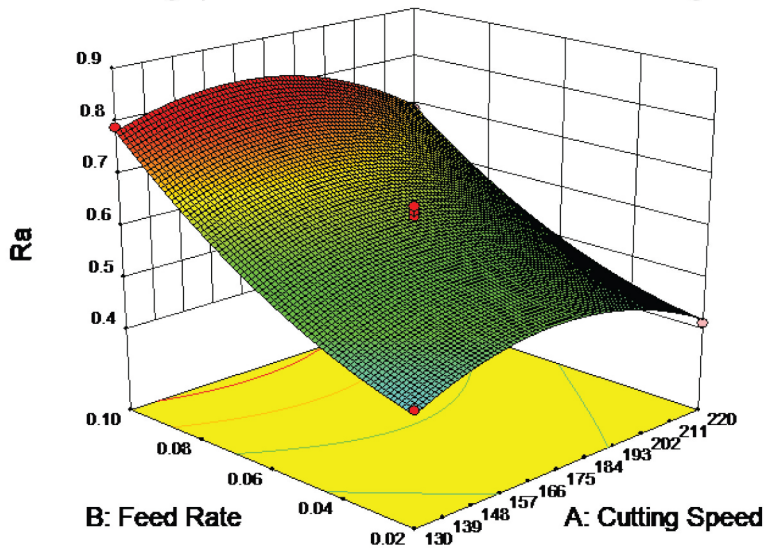
Effect of cutting speed and feed rate factors to surface roughness
