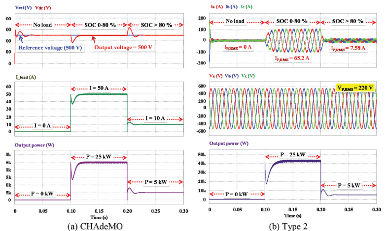
The operation of a fast electric vehicle battery charger (a) CHAdeMO (b) Type 2
