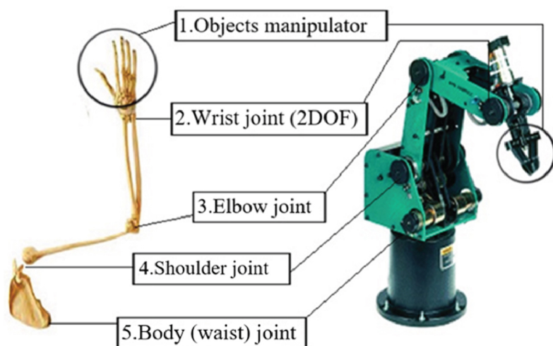
PC-Based 5DOF industrial robotic arm with object color sorting by image processing
