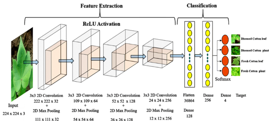
Figure 4 Convolutional Neural Network (CNN) Processes (Rai et al.).
