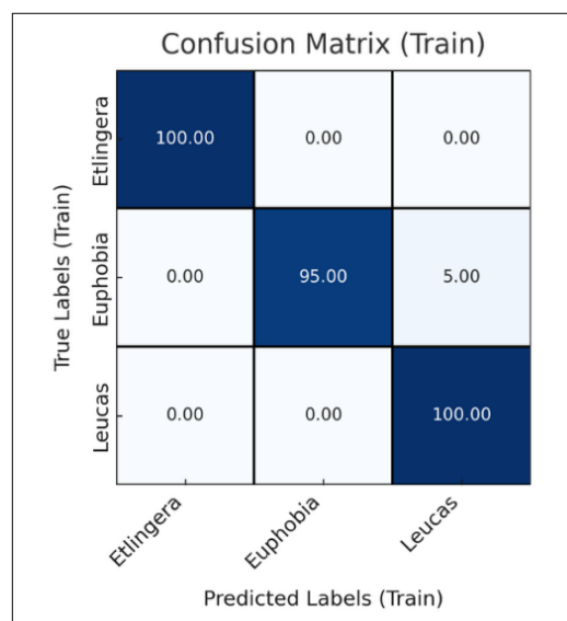
Figure 6 Confusion matrix training.
