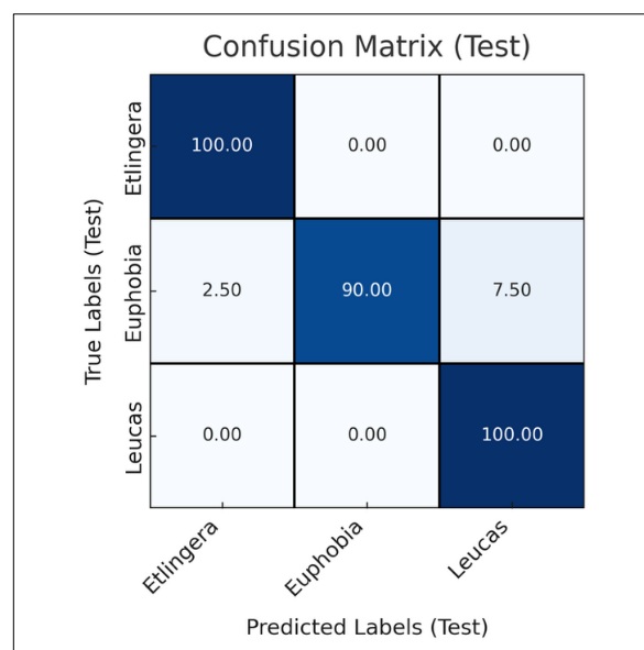
Figure 7 Confusion matrix testing.
