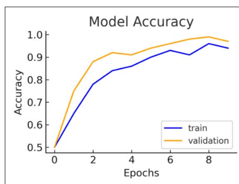
Figure 8 Model accuracy of training and validation over 10 epochs.
