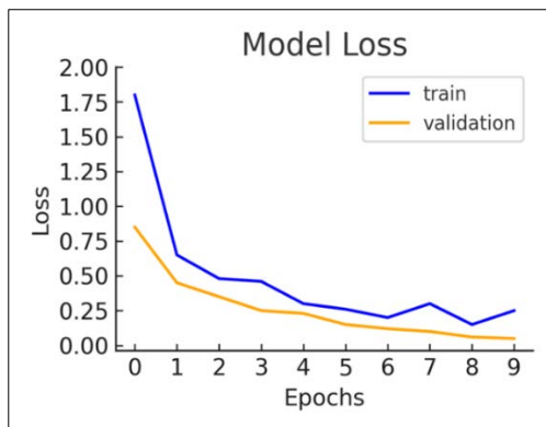
Figure 9 Model Accuracy of Training and Validation Over 10 Epochs.
