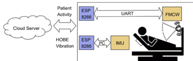
Figure 2 A framework of IoT-enabled nursing care bed.
