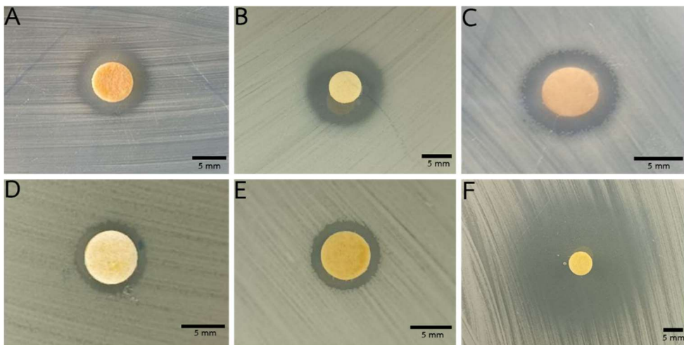
Figure 2 Antibacterial activity of lemongrass essential oil against extended-spectrum beta-lactamase (ESBLs) producer Gram-negative bacteria via disk diffusion method on MHA incubated at 37^{\circ}\text{C} for 18-24 h. (A) E. coli A3 -ESBLs, (B) S. aureus SP1, (C) P. aeruginosa A2 -ESBLs, (D) E. coli ATCC 25923, (E) K. pneumoniae A2 -ESBLs, (F) S. pyogenes SV1
