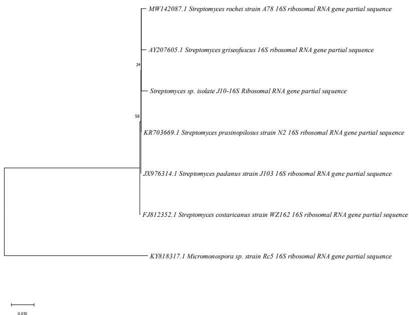
Figure 3 Phylogenetic tree of actinobacteria isolate J10 compared with Streptomyces spp. based on partial sequence of 16S rDNA gene.
