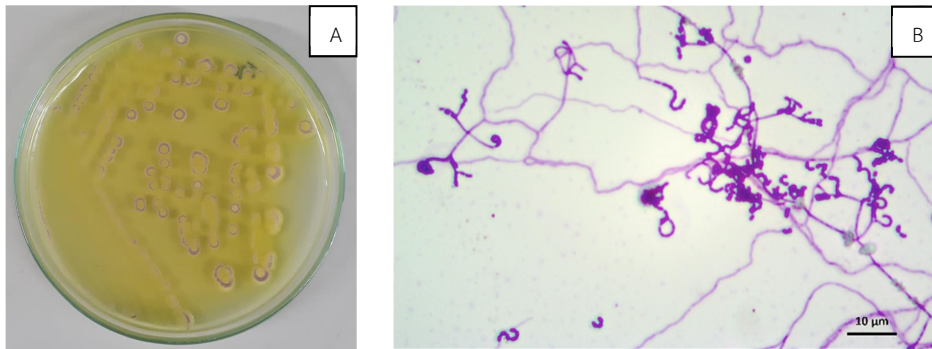
Figure 2 Characters of colony and conidia of actinobacteria isolate J10
