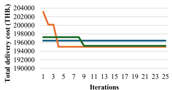
Figure 5 The total delivery cost of MPA, MMPA and MPA-GA (Example 1)
