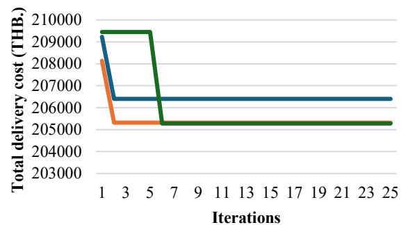
Figure 5 The total delivery cost of MPA, MMPA and MPA-GA (Example 1)
