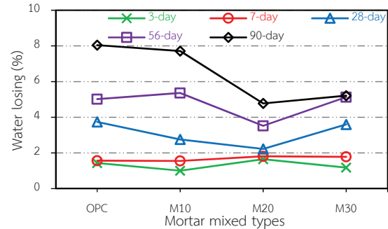
Figure 4 Water losing of mortar specimens blended with metakaolin at different ages.
