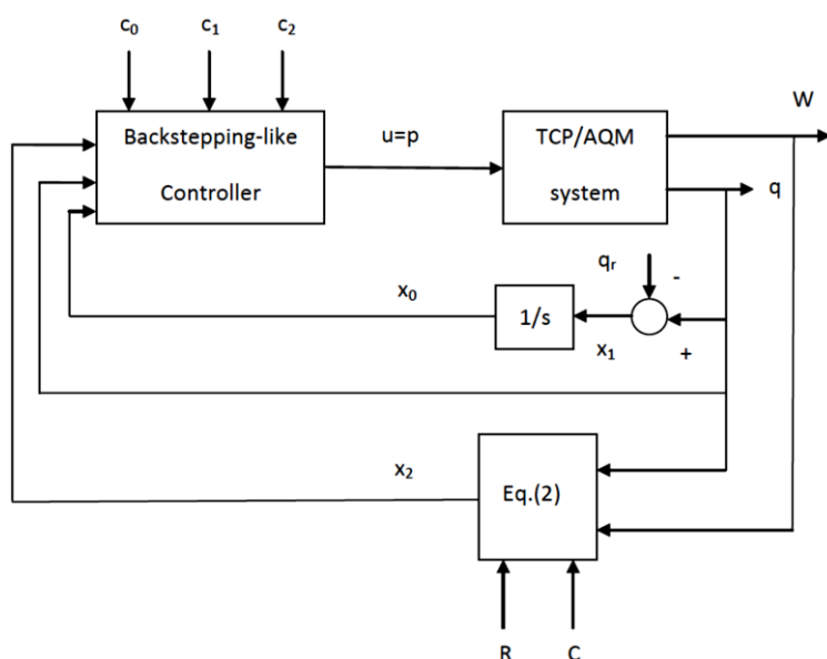
Figure 1 Block diagram of the proposed backstepping strategy for the TCP/AQM system.
