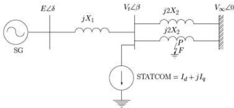
Figure 1 A single line diagram of the SMIB model with STATCOM
