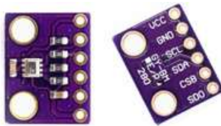
Figure 5 BM280 pressure sensor for measuring altitude
