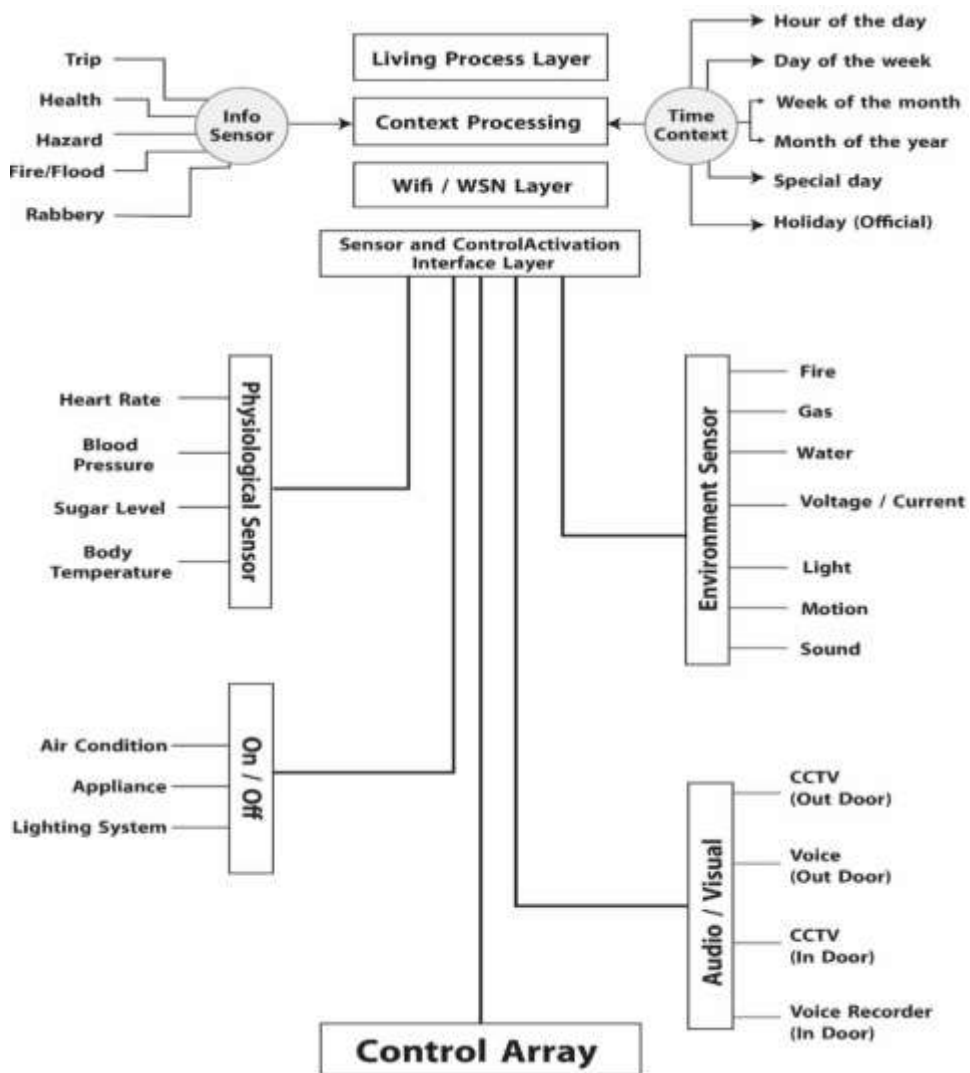
Figure 4 Architecture of Context-aware Living Process Smart Home.
