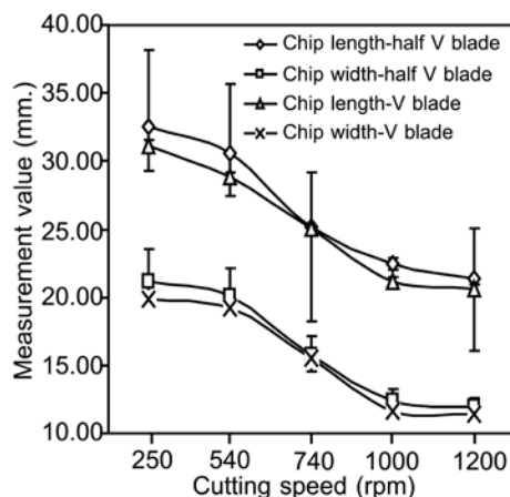
Figure 6 Relation of chip size, cutting speed, and blades
