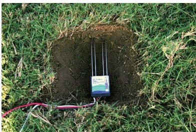
Figure 5 Soil Moisture Sensor, EC (pH) Sensor and Solenoid water valve installation
