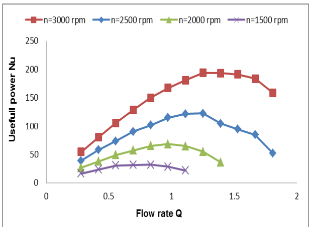
Fig. 5. Shows the curve Result of Water horse power vs Discharge at different rotational speed.
