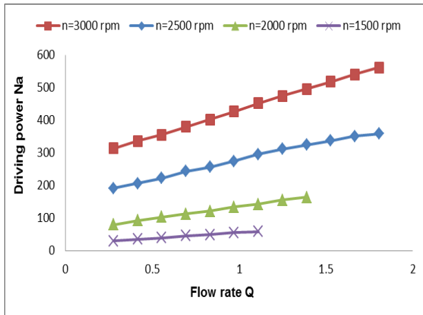
Fig. 6. Shows the curve Result of Input horse power vs Discharge at different rotational speed.
