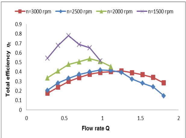
Fig. 7. Shows the curve Result of pump efficiency vs Discharge at different rotational speed.
