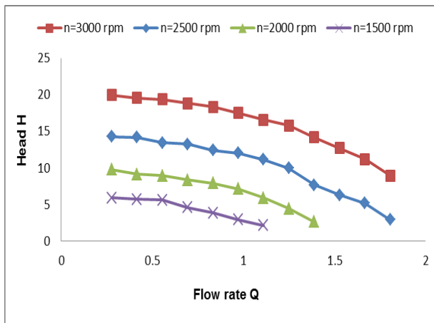
Fig. 4. Shows the curve Result of Head vs Discharge at different rotational speed.
