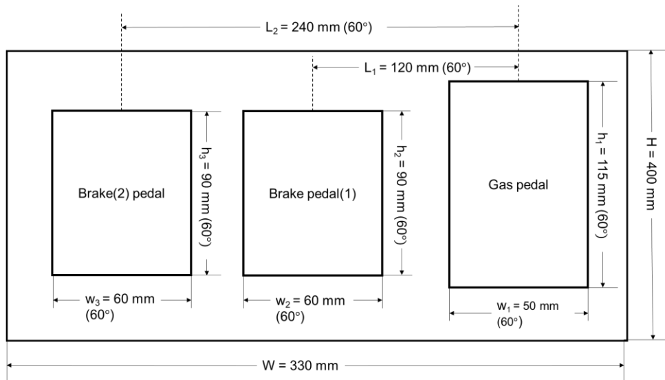
Fig. 4. Arrangement and dimensions of brake and gas pedals.
