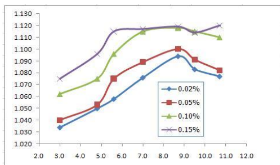
Fig. 3 Effect of pH on thermal conductivity of Al 2 O 3 -H 2 O suspensions
