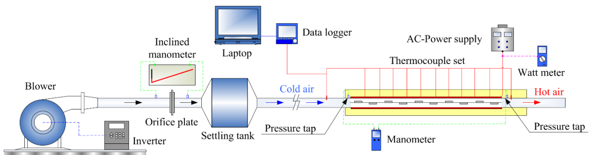
Fig. 1. Schematic diagram of the experimental setup.
