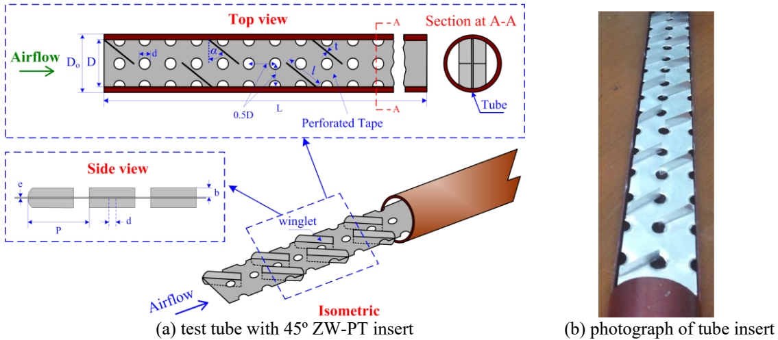
Fig. 2. The ZW-PT arrangements used in the present work.
