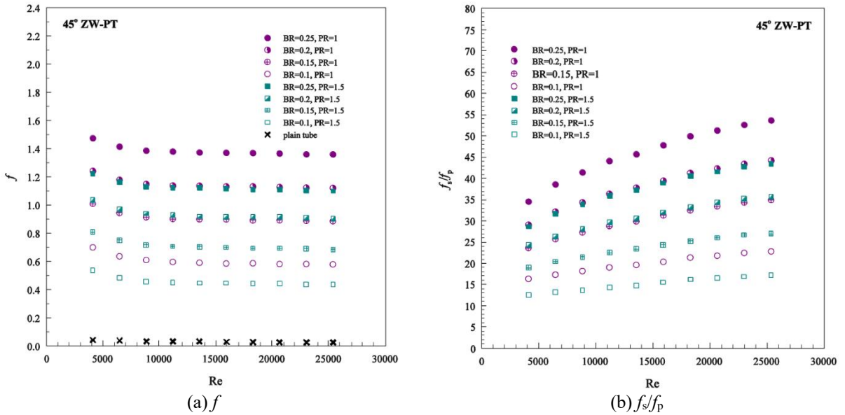
Fig. 5. Variation of f and f_s/f_p with Re for ZW-PT insert.
