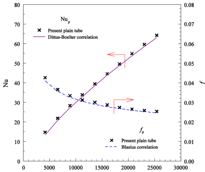
Fig. 3. Verification of Nu and f for plain tube.
