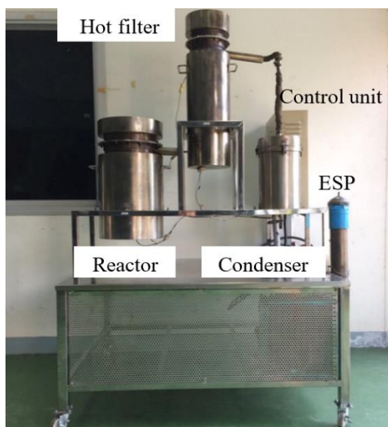
Plastic pyrolysis
