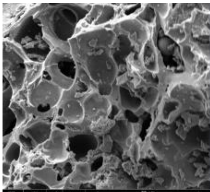
SEM micrographs of activated carbon from longan seeds
