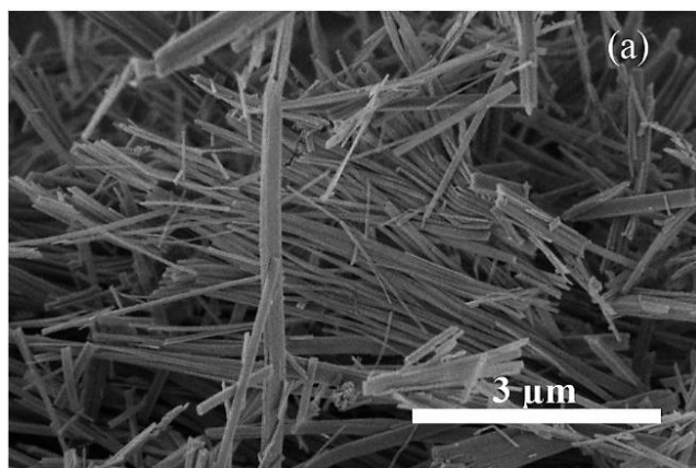
TiO 2 nanowire by Ni with hydrothermal method
