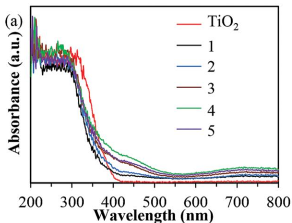
TiO 2 nanowire by Ni with hydrothermal method
