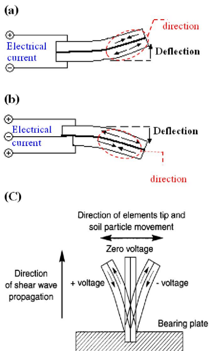
Fig. 2. Overview of bender elements (BE): (a) Connection of BEs by series type, (b) Connection of BEs by parallel type and (c) Mechanism of BEs generating S-wave by supplying electrical current adapted from [25, 30, 32].
