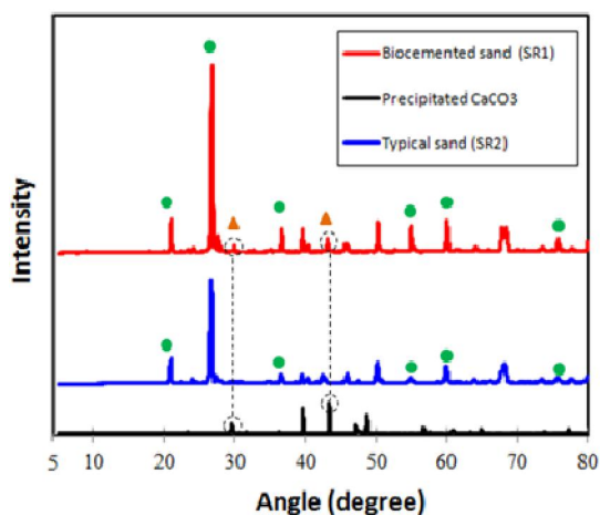
Fig. 5. Pattern differences of X-ray diffraction between typical sand and treated sand after biocementation
