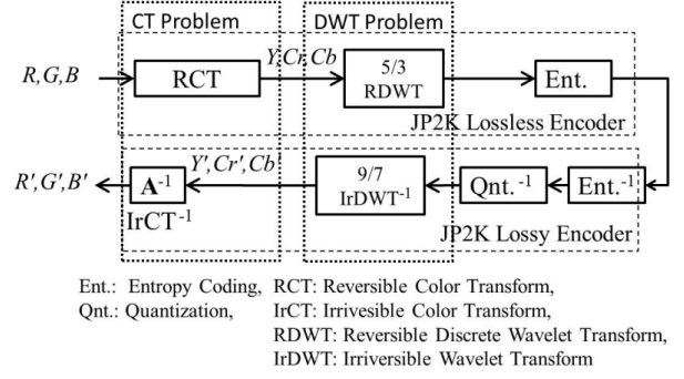
Fig.2: Compatibility Problem of Lossless-Lossy coding.
