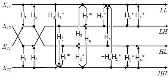
Fig.15: Non-scaled NS 9/7 RDWT.
