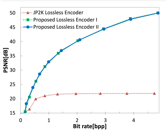
Fig.17: 1 st Stage RDWT on Proposed Lossless Encoder.
