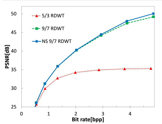
Fig.11: 1 st Stage comparison of 3 RDWT.
