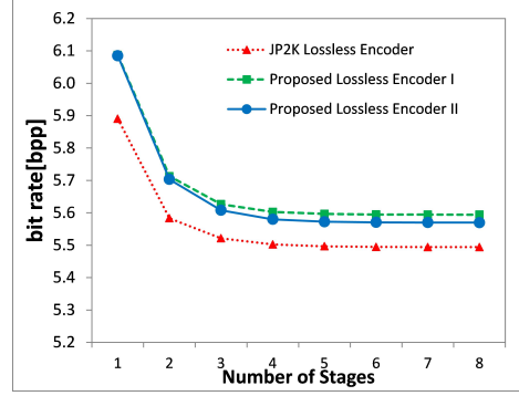
Fig.25: Average bit rate in Mandrill image.
