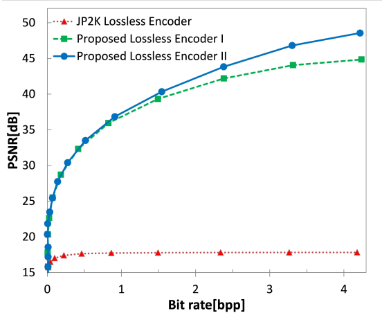
Fig.19: Comparison of Proposed Lossless Encoder.
