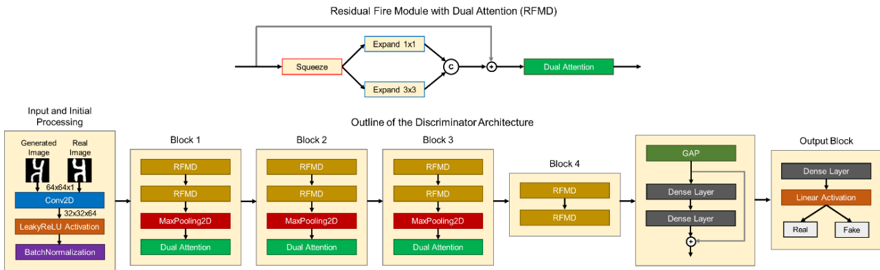
Figure 4 An outline of the proposed Discriminator architecture.
