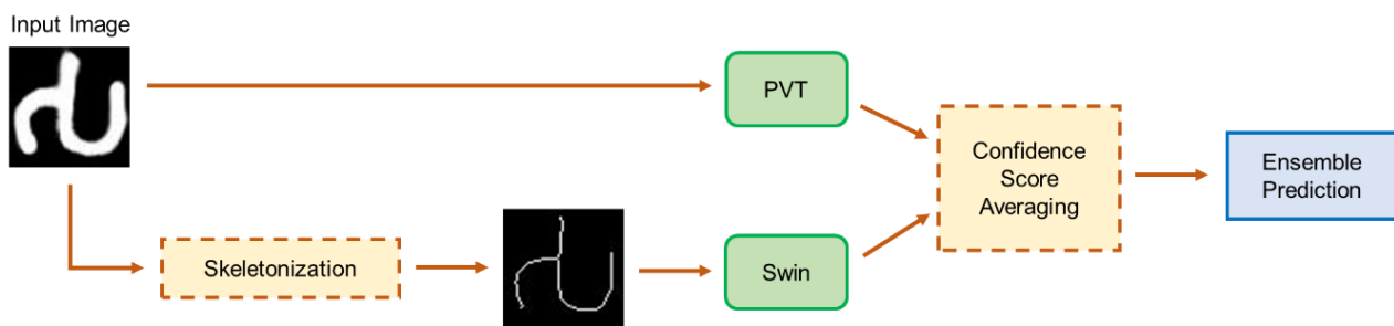
Figure 5 An outline of the ensemble prediction model.
