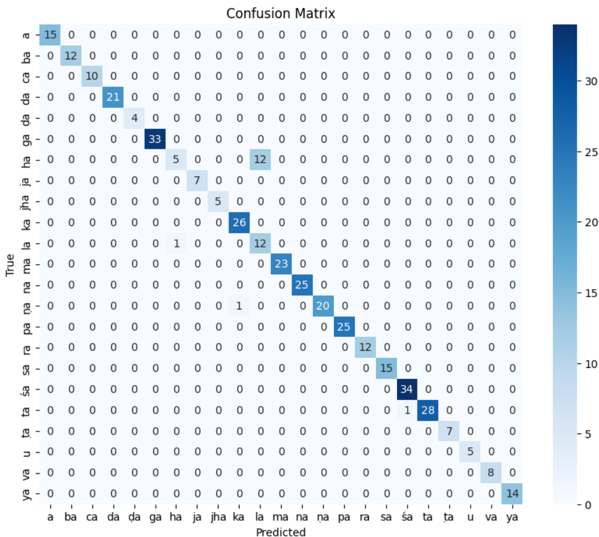
Figure 8 Confusion matrix of the proposed ensemble Transformer classifier on real test images.
