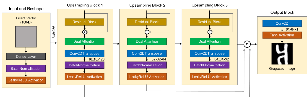
Figure 3 An outline of the proposed Generator architecture.
