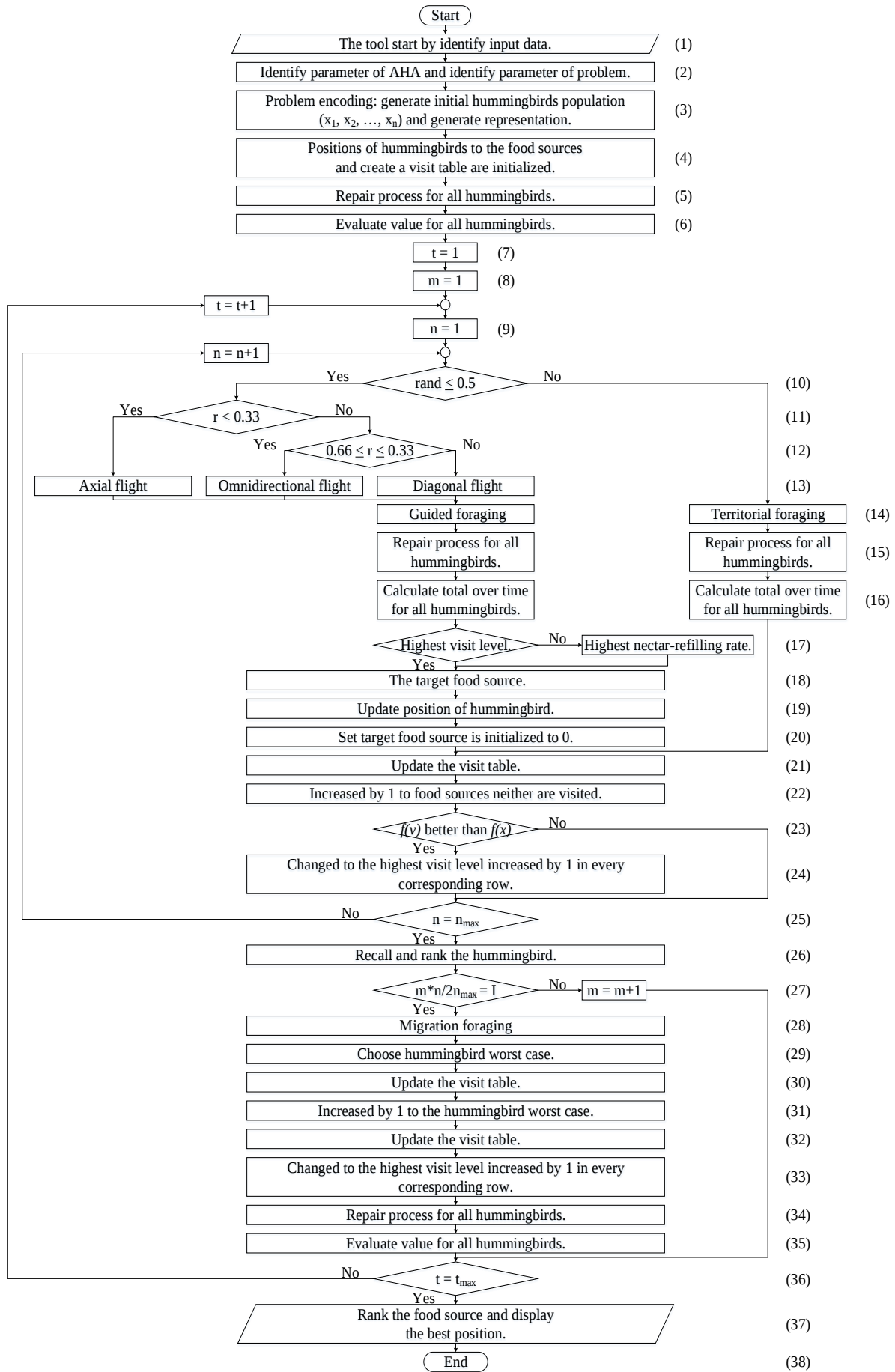
Figure 7 Flowchart of the AHA scheduling tool
