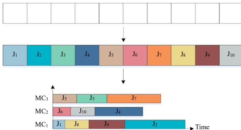
Figure 8 Example of a single solution
