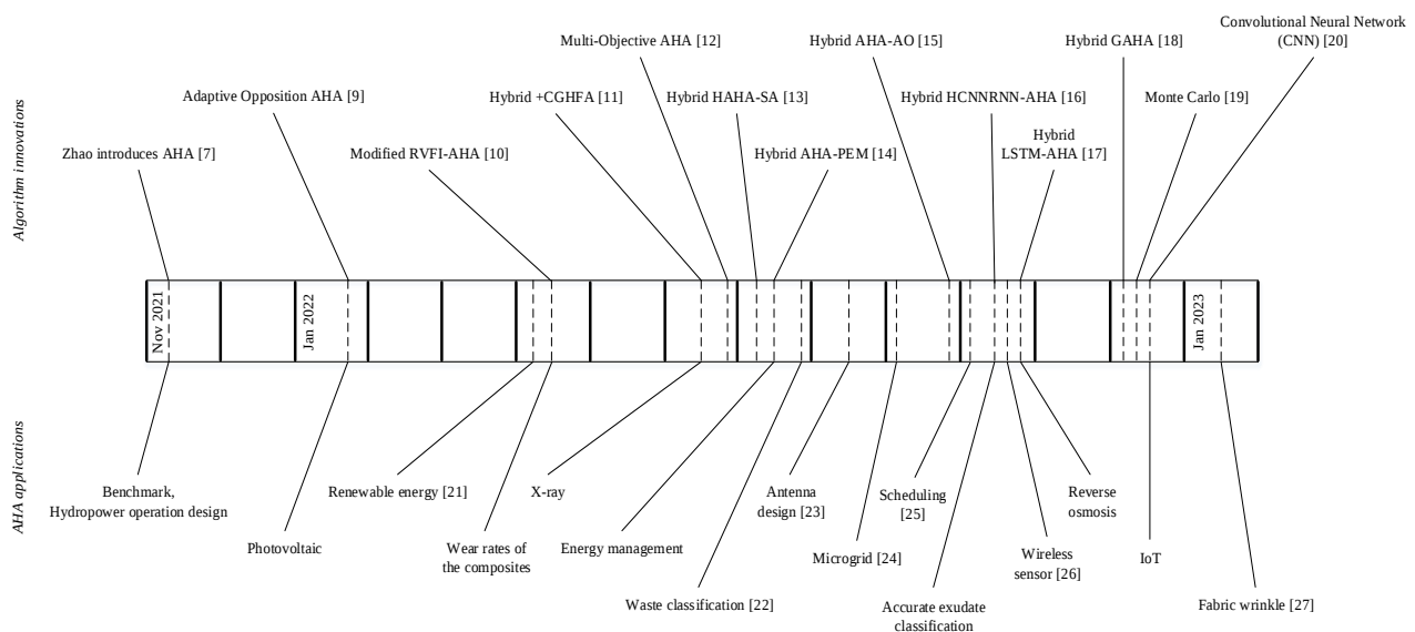
Figure 1 Chronology of selected developments and applications of the AHA from 2021 to 2023
