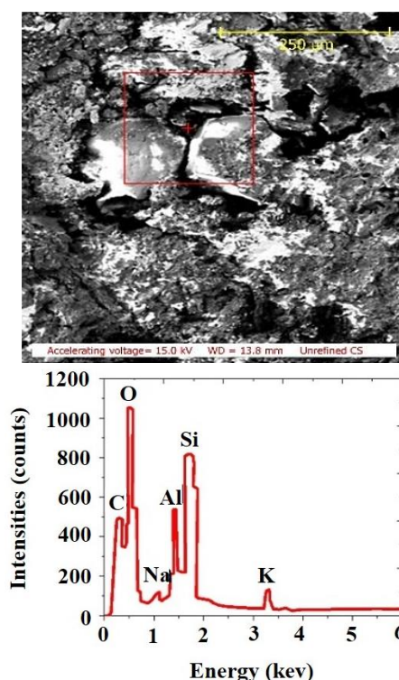
Figure 1 SEM/EDX showing the structural morphology of unrefined coconut shell and elemental composition of the coconut shell at the analysed area
