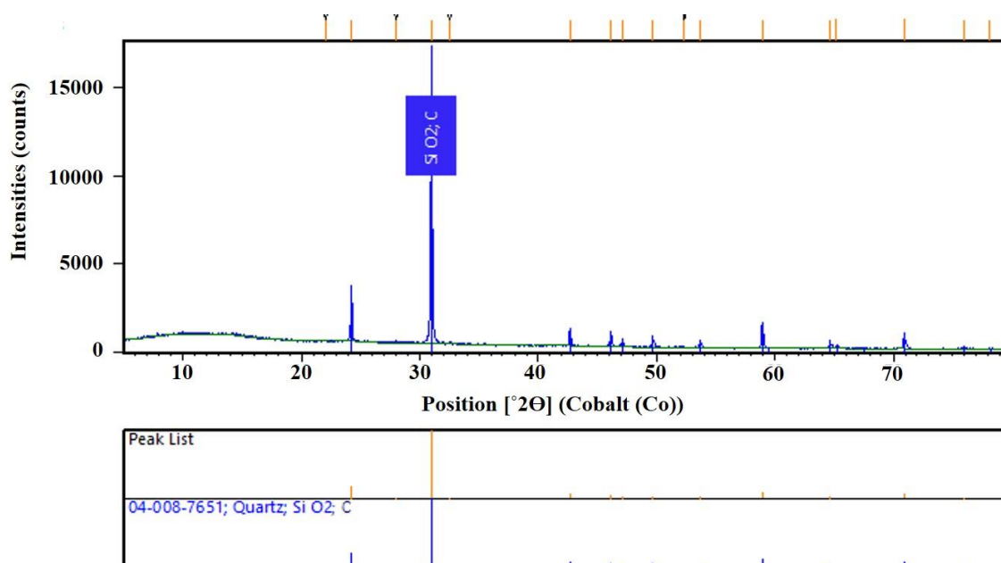
Figure 9 X-ray diffractometric properties of uncarbonised coconut shell nanoparticles obtained by milling for 70 hours at a CR value of 20 showing phases at different diffraction angles, 2θ
