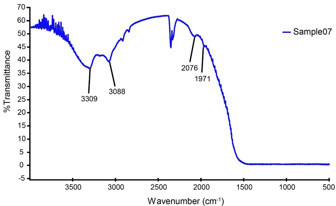
Figure 4. Mid-IR absorption spectrum of boehmite/diaspore in a Longido ruby (sample no. 07) showing peaks at 1971, 2076, 3088 and 3309 cm -1 .
