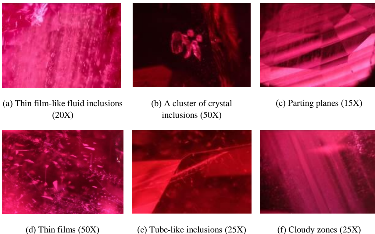
Figure 2. Different types of inclusions in rubies from Longido, Tanzania. Photomicrographs by M.Maneeekrajangsaeng and S. Promwongnan.
