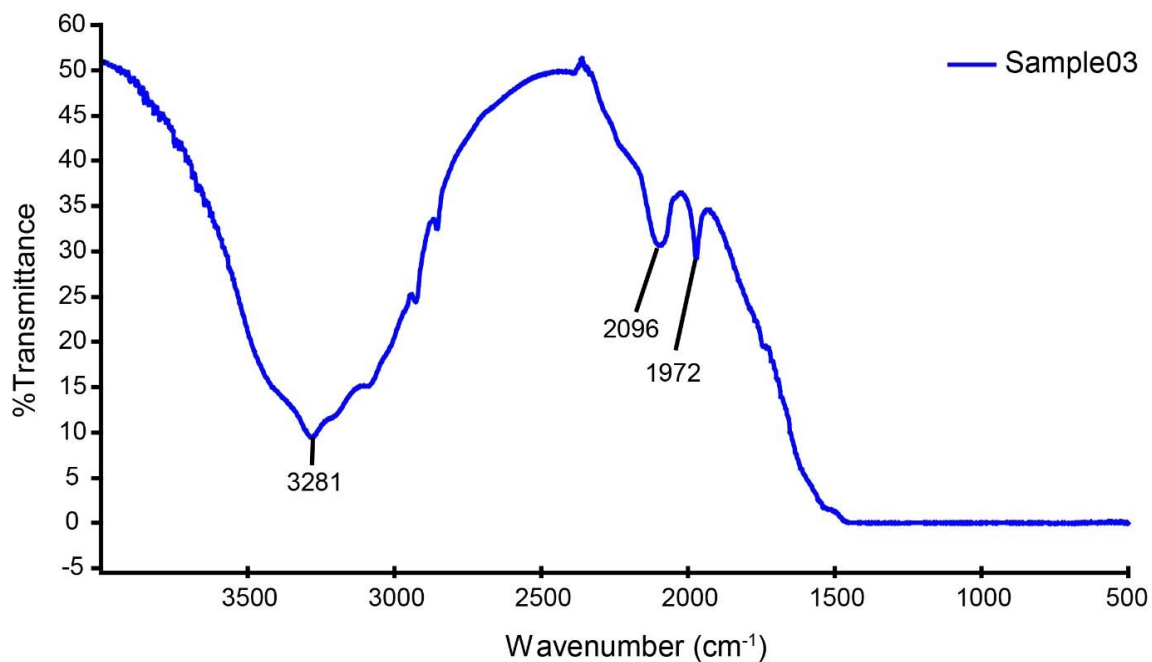
Figure 3. Mid-IR absorption spectrum of boehmite/diaspore in a Longido ruby (sample no. 03) showing peaks at 1972, 2096 and 3281 cm -1 .
