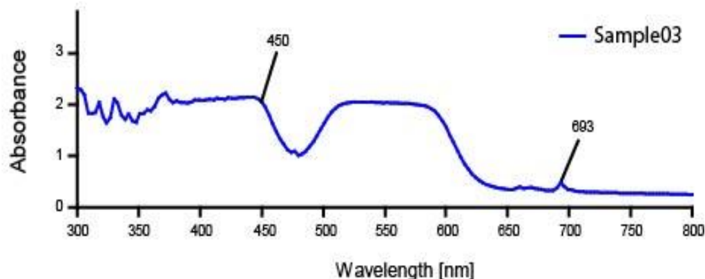
Figure 5. A representative non-polarized UV-Vis-NIR absorption spectrum of a Longido ruby (Sample no. 03).
