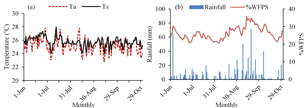
Figure 3 Graphs of (a) Air temperature (Ta), soil temperature (Ts) and (b) total monthly rainfall and soil moisture from June to October 2016.
