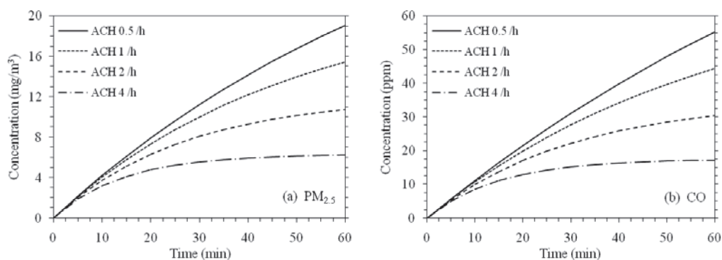
Figure 3 Predicted time-dependent concentrations when burning three incense sticks and one candle in a room with four different air exchange rates for (a) PM 2.5 and (b) CO.
