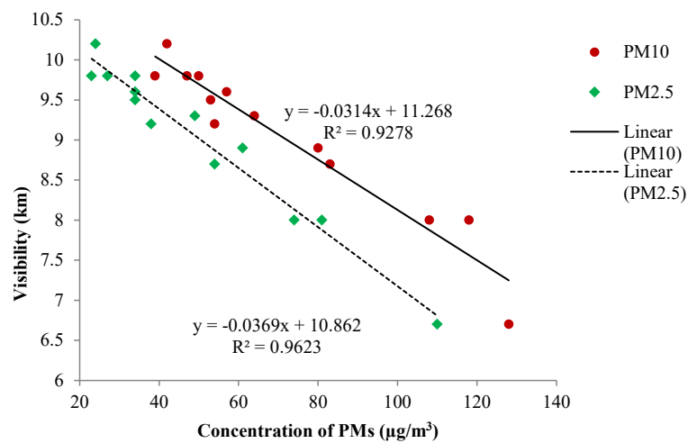
Figure 7 Visibility correlation with PM 10 and PM 2.5 data from the Meteorological Station 2015-2016 (N18.47240, E98.58370) at altitude 313 m.
