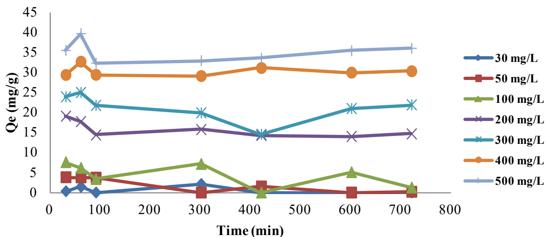
Figure 4 Effect of initial MH concentration on PAAC removal
