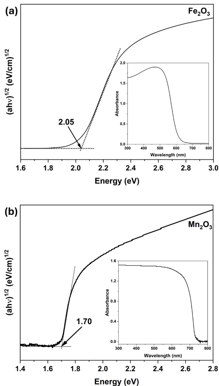
Supplementary Figure 1 DRS results of (a) Fe 2 O 3 and (b) Mn 2 O 3 samples.
