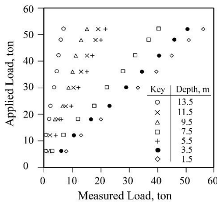
Figure 11 Applied load versus measured load from gauges in steel pile E
