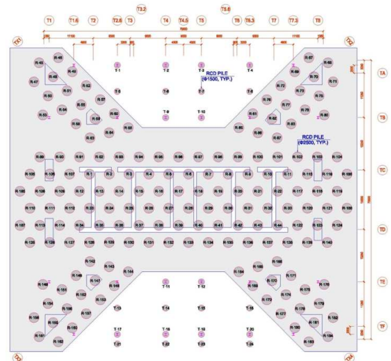
Figure 7. Pile Layout Plan
