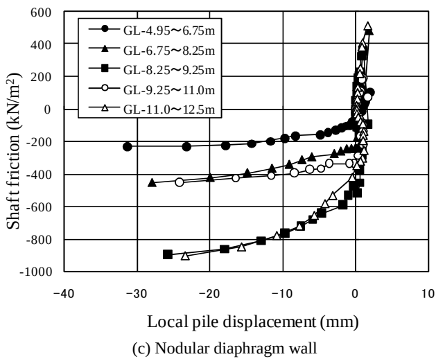
Figure 10 Relationships between shaft friction and displacement
