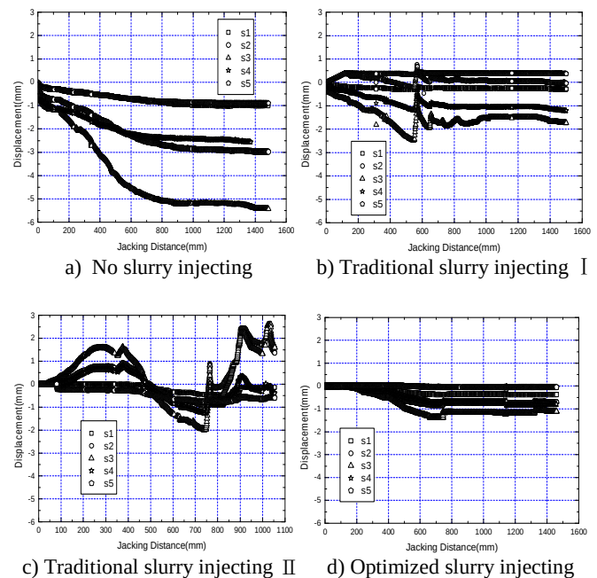
Figure 9 Ground settlements changing with the advancing distance of 4 conditions
