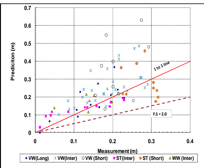
Figure 22. Prediction by Eq. (24) vs. Sturm's abutment scour database (2004)
