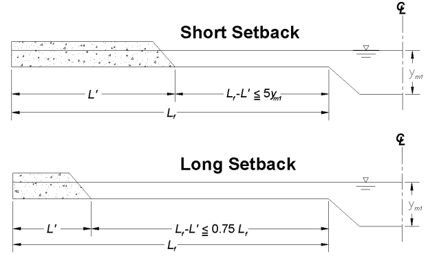
Figure 7. Definition of degree of setback.
