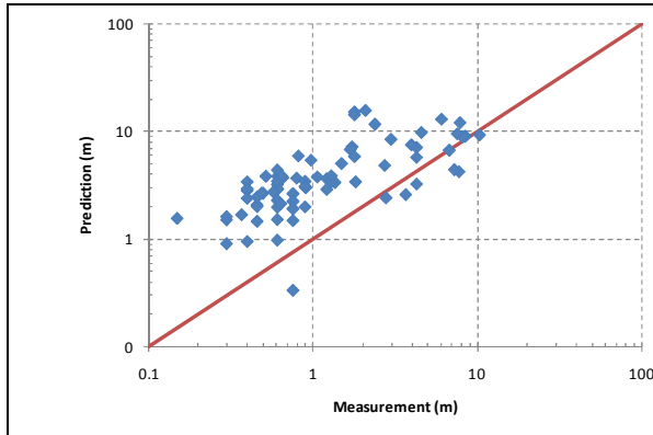
Figure 17. Prediction by Eq. (8) versus Froehlich's pier scour data base (1988)
