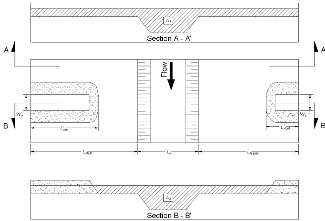
Figure 11. Definition of parameters in the contraction scour
