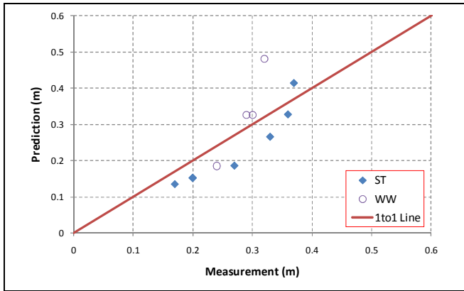
Figure 23. Prediction by Eq. (24) vs. Ettema et al.'s abutment scour database (2008)
