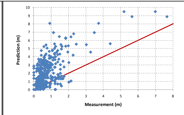
Figure 18. Prediction by Eq. (8) versus Muller and Landers' pier scour database (1996)
