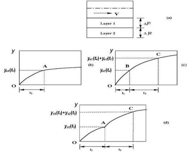
Figure 10. Scour on multi-layers
