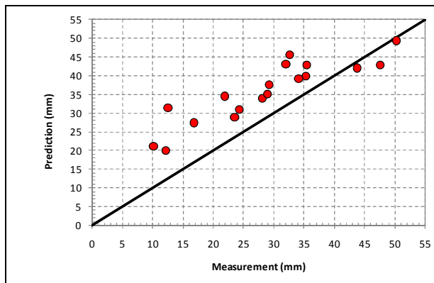
Figure 19. Prediction by Eq. (15) vs. Gill's contraction scour database (1981)
