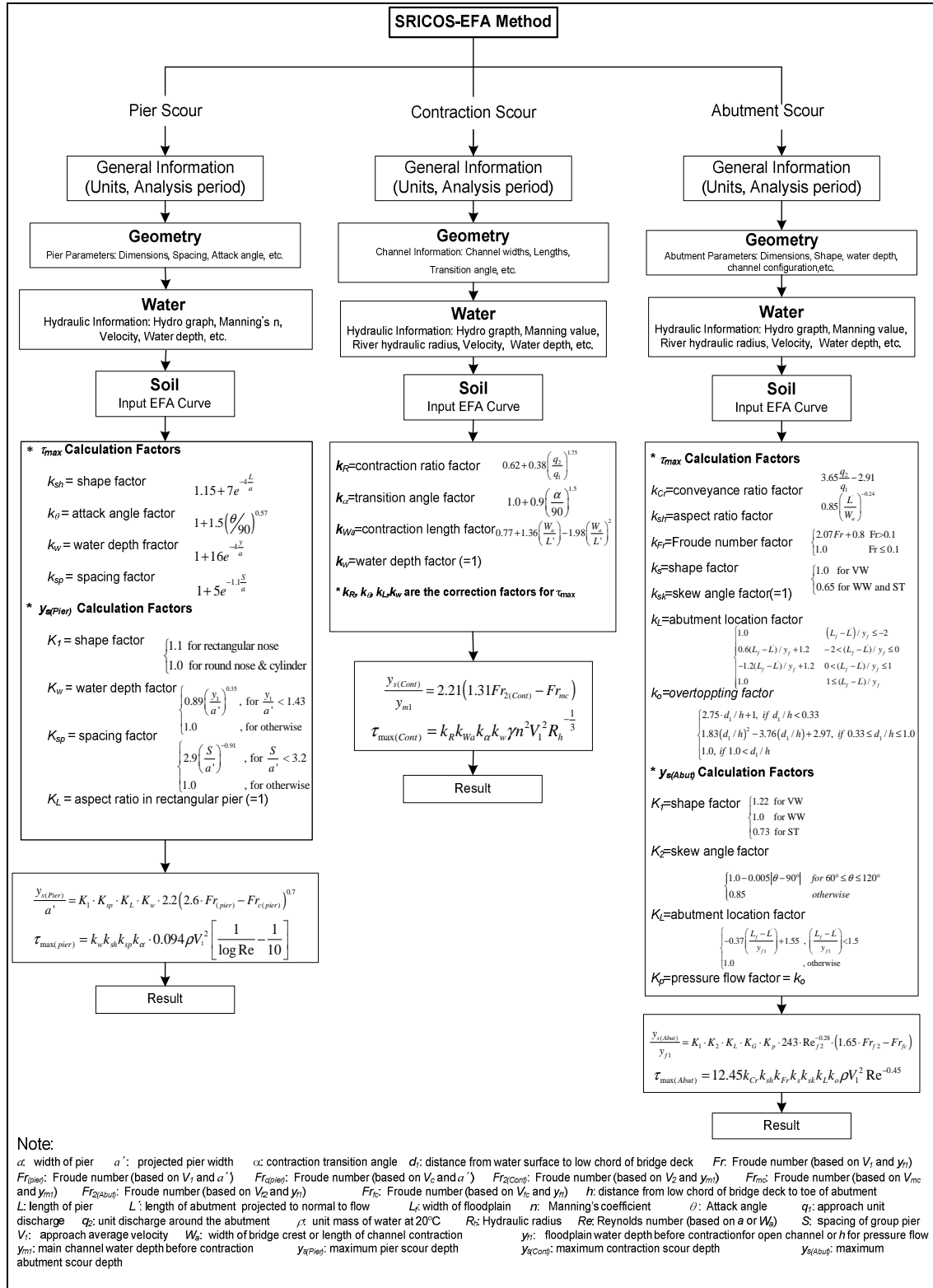
Figure 12. Procedure of SRICOS-EFA method
