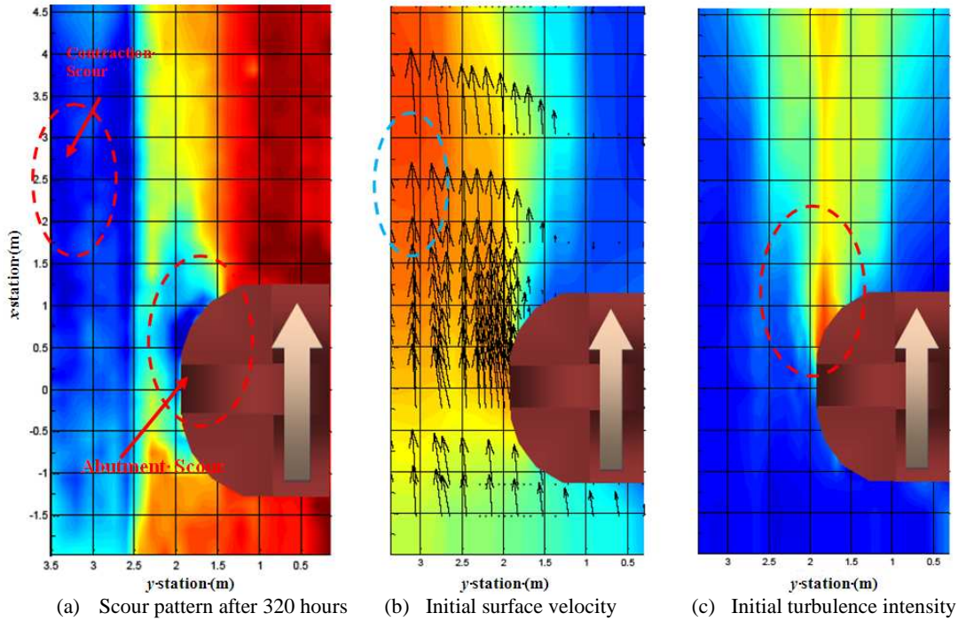
Figure 6. Comparison of scour pattern and velocity pattern (Oh, 2009)
