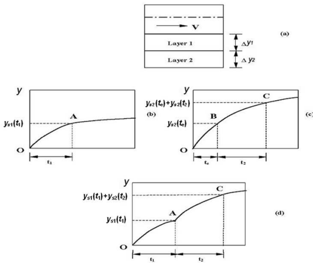
Figure 9. Scour due to a sequence of two flood events
