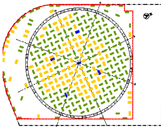
Figure 12. ICC Tower-Foundation plan
