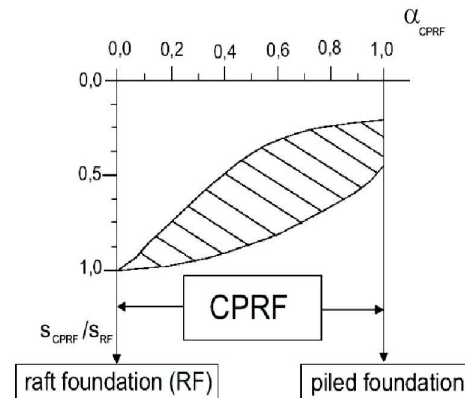
Figure 9. Settlement ratio \xi_7 versus \alpha_{CPRF} .
