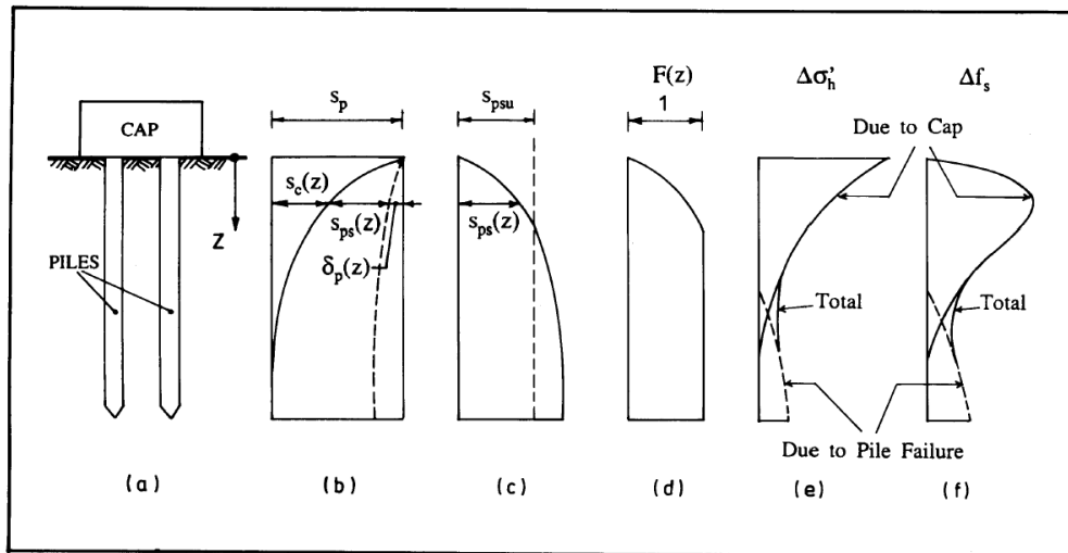
Figure 7. Increase in skin friction along a pile, due to effect of cap being in contact with soil surface and effect of failure zone at pile base, Phung (1993).
