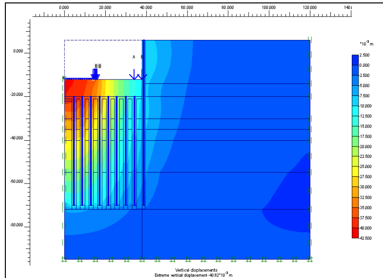
Figure 11. ICC Tower-Axisymetrical modelling foundation using Plaxis, Phung (2002)
