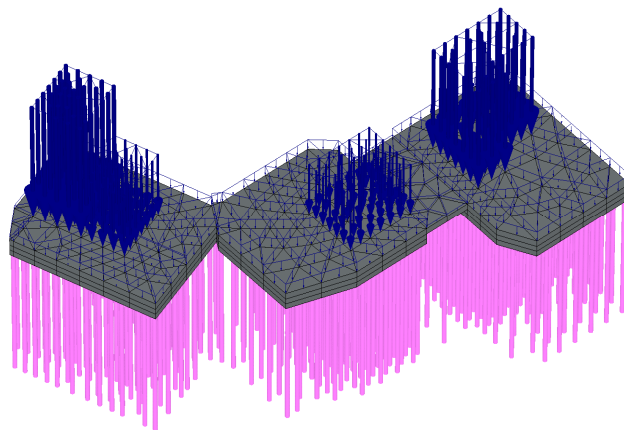
Figure 14. 3D-Modelling a piled-raft using Plaxis 3D Foundation –Vers 2. (Brikgreve, 2008)
