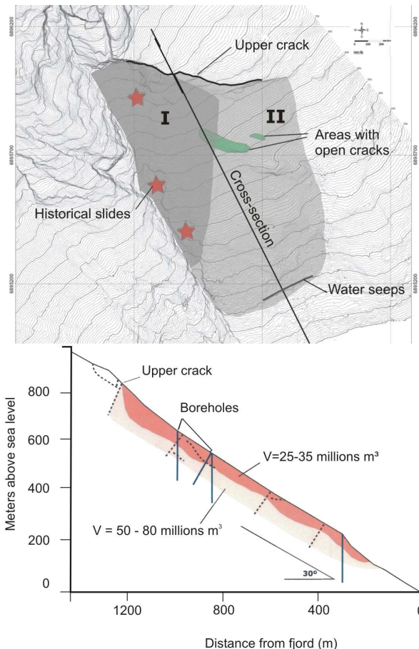
Figure 12. Sliding volume scenarios. Surficial area (top) and cross-section (bottom) (modified from Blikra et al. 2007)
