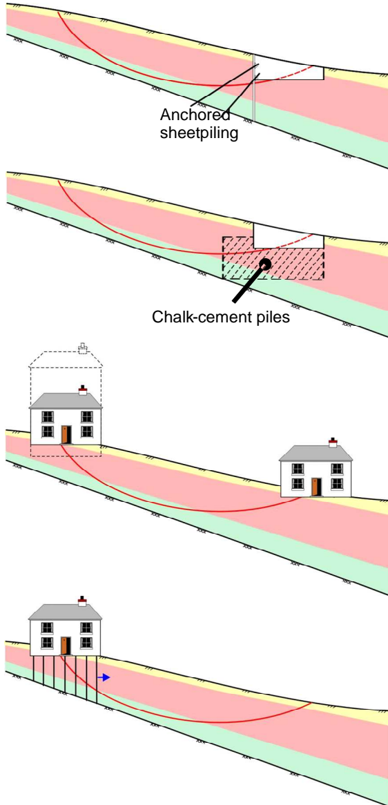
Figure 10. Hazard, mitigation and preventive measures in Zone II in Drammen (Gregersen, 2008; Karlsrud, 2008)
