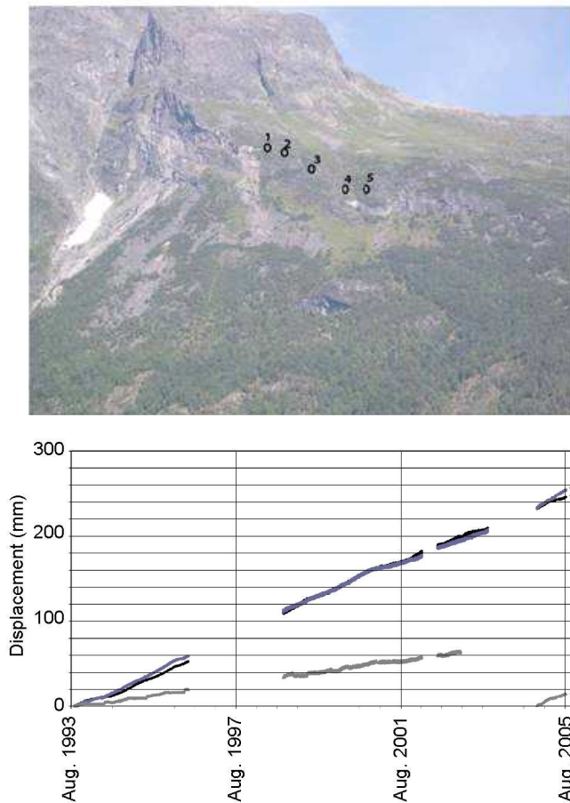
Figure 13. Location of extensometers and displacements from extensometer 1, 2, 3, 4 and 5 at the top scarp at Åknes (Kveldsvik et al. 2006)
