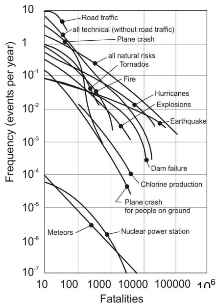
Figure 3. F-N curves (Proske, 2004)
