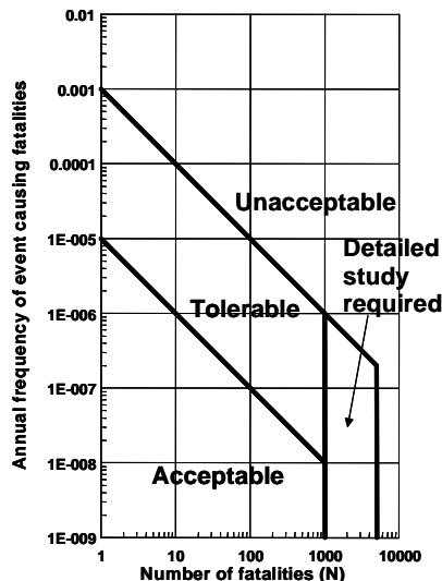
Figure 4. Hong Kong criteria (GEO, 1998)
