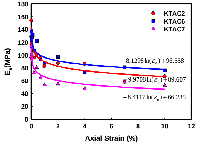
Figure 20 Relationship between E_e and axial strain for anisotropically consolidated specimens.
