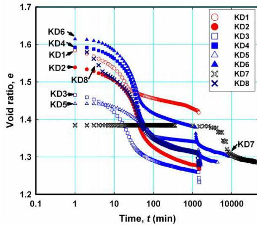
Figure 5 Variation of void ratio, e , with time during consolidation as examined in DSB tests.
