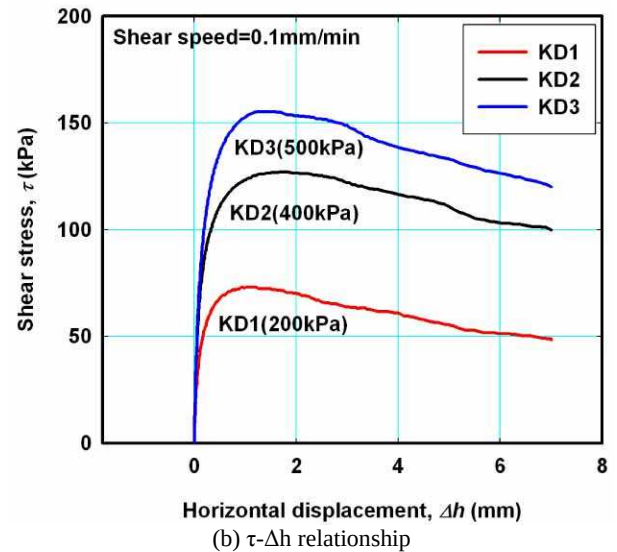
Figure 8 Results of constant-volume DSB tests with the horizontal displacement rate of 0.1mm/min.
