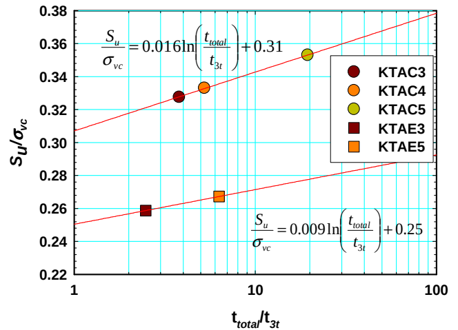
Figure 11 Effects of consolidation time on s_u/\sigma_{vc} in a series of triaxial tests
