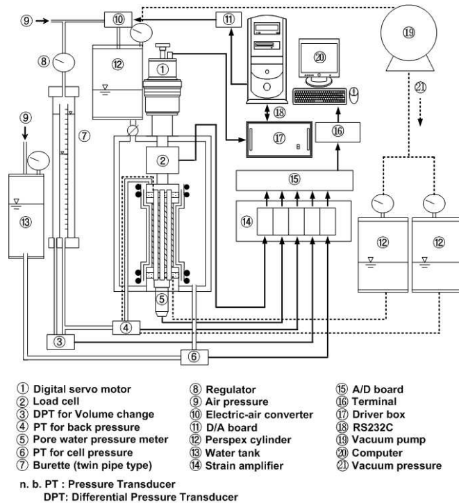
Figure 1 Triaxial apparatus employed.
