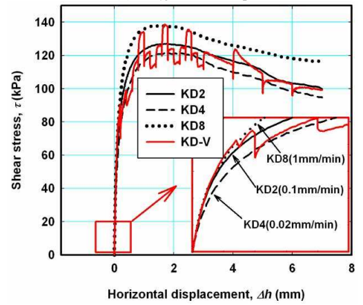
(b) \tau - \Delta h relationship
