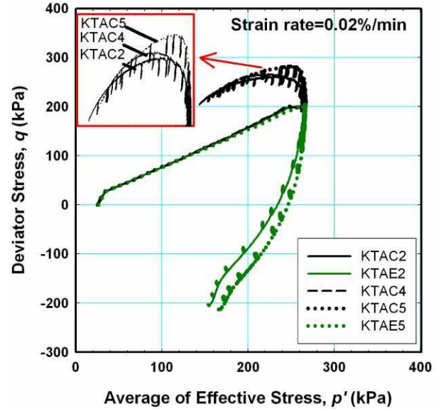
Figure 10 Undrained effective stress paths of a series of triaxial tests using different consolidation periods.
