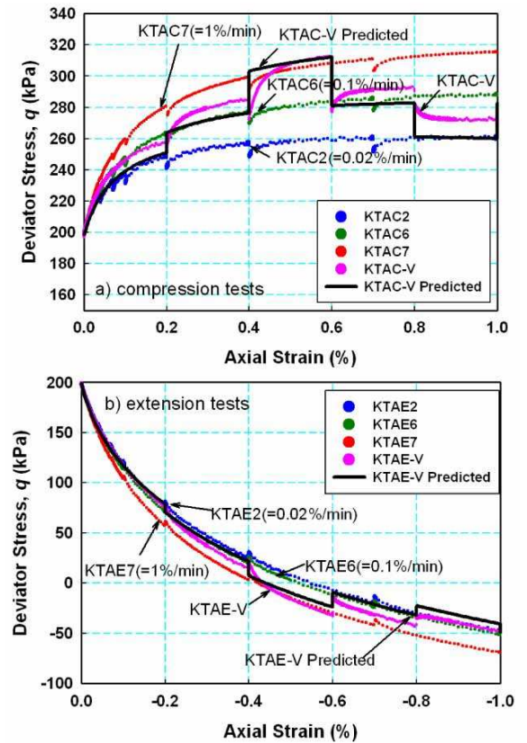
Figure 26 Predicted versus measured relationship between deviator stress and axial strain ( \epsilon \leq 1\% for anisotropically consolidated specimens).
