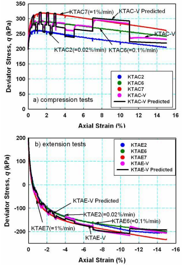
Figure 25 Predicted versus measured relationship between deviator stress and axial strain (full range of \epsilon for anisotropically consolidated specimens).
