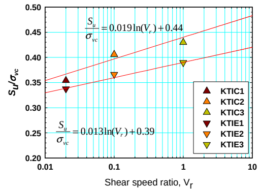
b) Triaxial test(isotropically consolidated)
