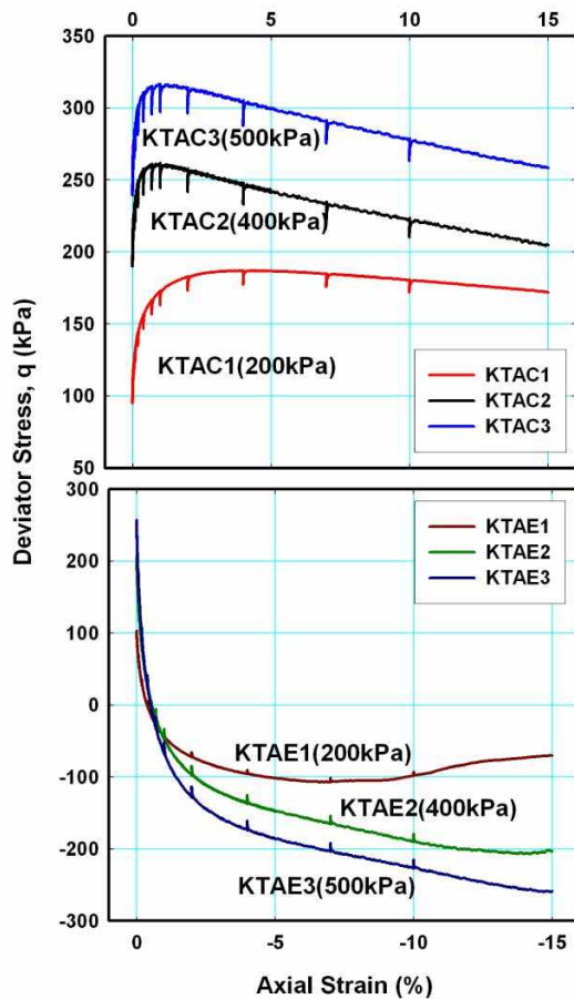
Figure 6 Stress-strain relationship of a series of triaxial tests using the axial strain rate of 0.02 %/min
