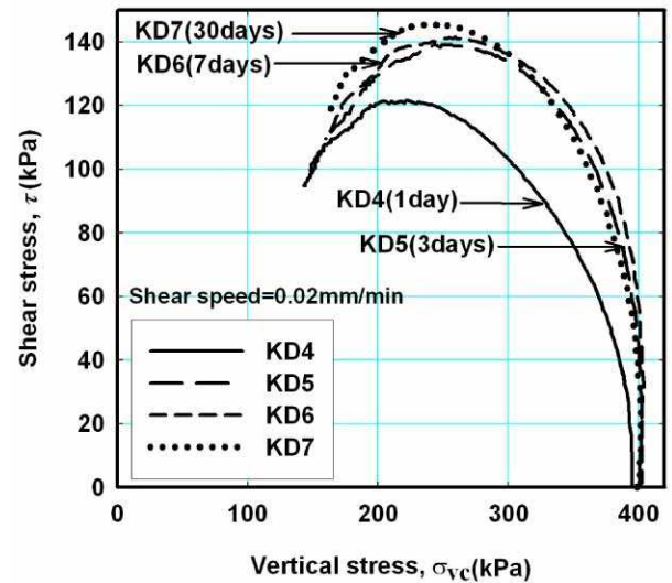
(a) \tau - \sigma_{vc} relationship
