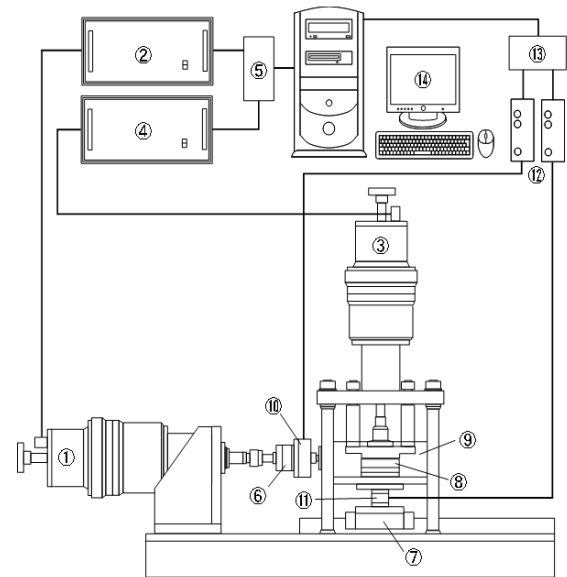
①:direct drive motor for lateral loading ②:drive unit for lateral loading ③:direct drive motor for vertical loading ④:drive unit for vertical loading ⑤:serial correspondence board ⑥:slide unit ⑦:linear roller way ⑧:shear box ⑨:outer box ⑩:load cell for lateral loading ⑪:load cell for vertical loading ⑫:strain amplifier ⑬:AD transformation board ⑭:personal computer
