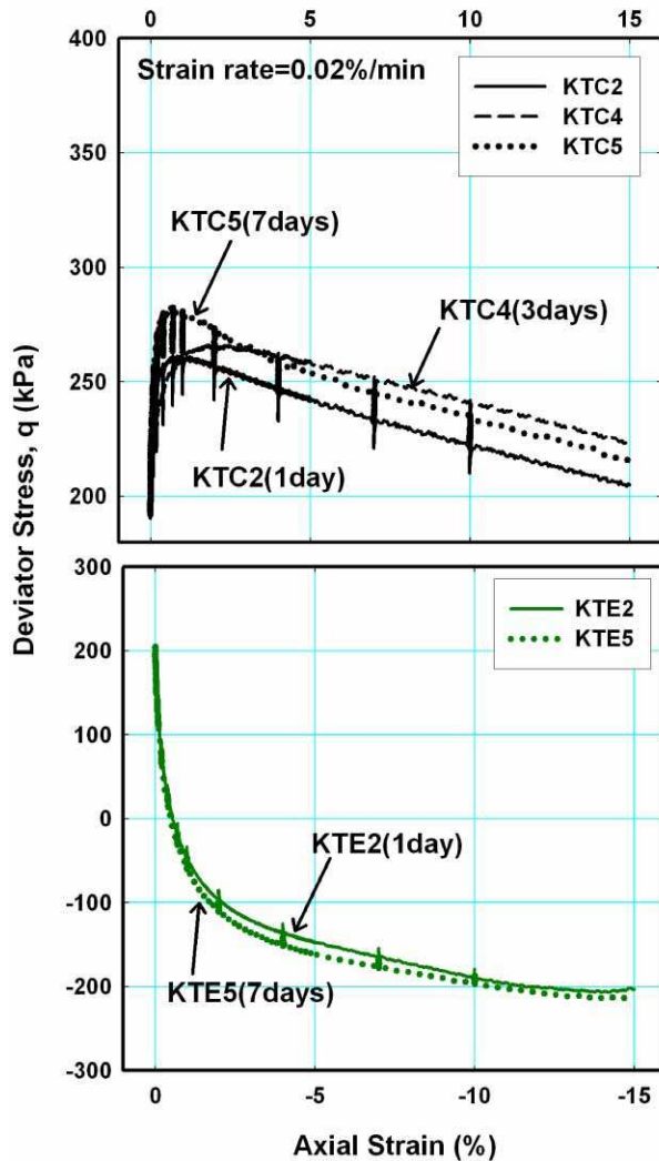
Figure 9 Stress-strain relationship of a series of triaxial tests using different consolidation times.
