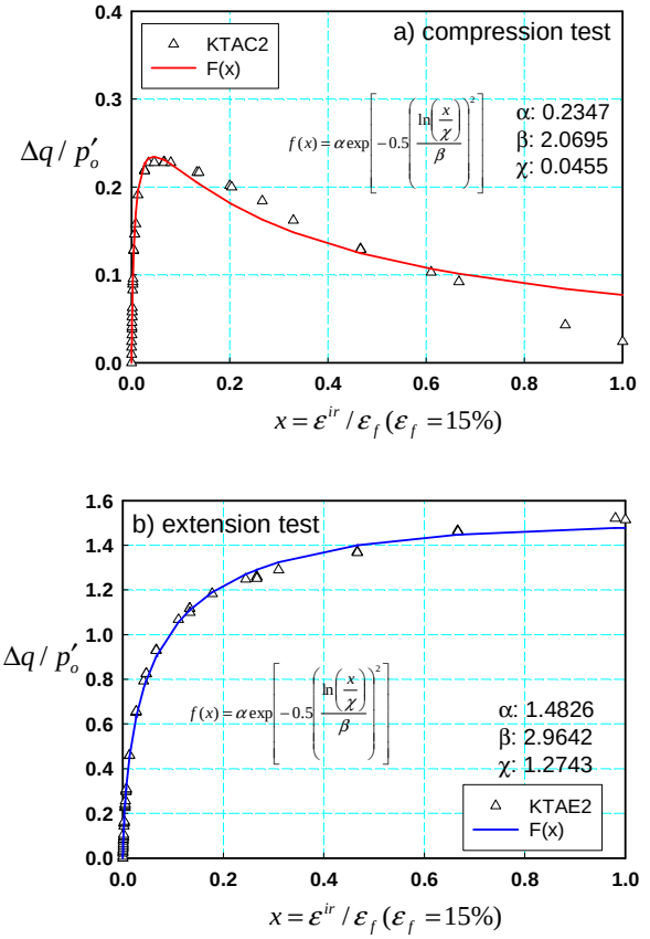
Figure 21 Shape function in the isotach model proposed (anisotropically consolidated specimens).
