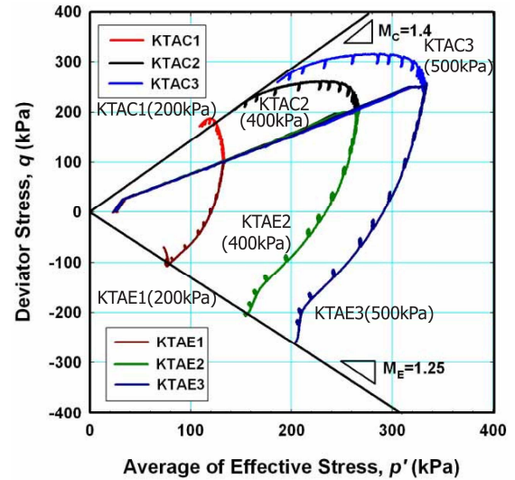
Figure 7 Undrained effective stress paths of a series of triaxial tests using the axial strain rate of 0.02 %/min
