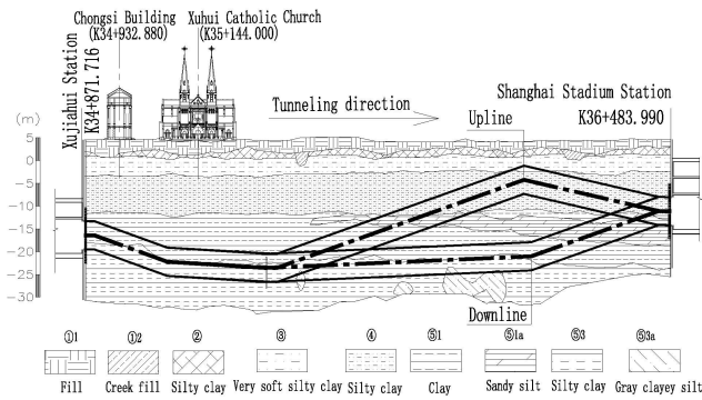
Figure 1 Soil profile and the location of tunnels
