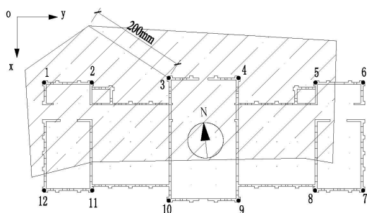
Figure 7 Comparison of the original building outline and the outline after deformation
