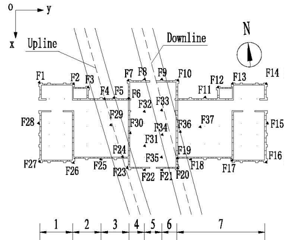
Figure 12 Plan of monitoring points of Chongsi Building
