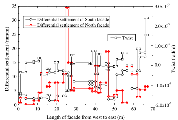
Figure 9 Original differential settlement and Twist of Chongsi Building
