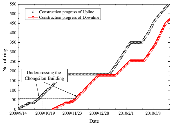
Figure 10 Construction progress of shield tunnels crossing historic buildings
