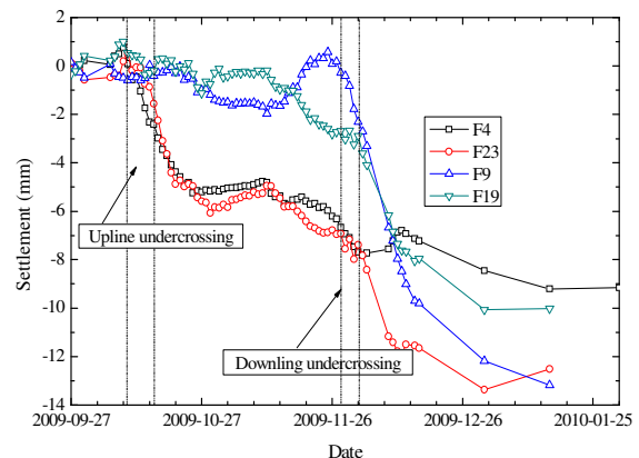
Figure 14 Settlement development with the construction process for some key measuring points
