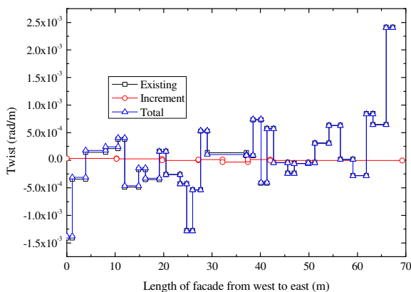
Figure 18 Comparison of existing, incremental and total twists of Chongsi Building
