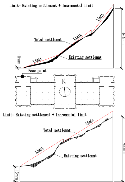
Figure 17 Comparison of existing, total settlements and incremental limit of Chongsi Building
