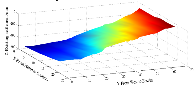
Figure 8 Relative height of bottom windowsill (unit: mm)
