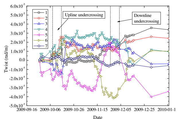
Figure 15 Development of twist with the construction process
