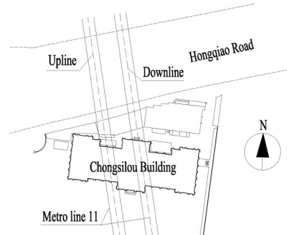
(a) Plan view of the tunnels and Chongsi Building
