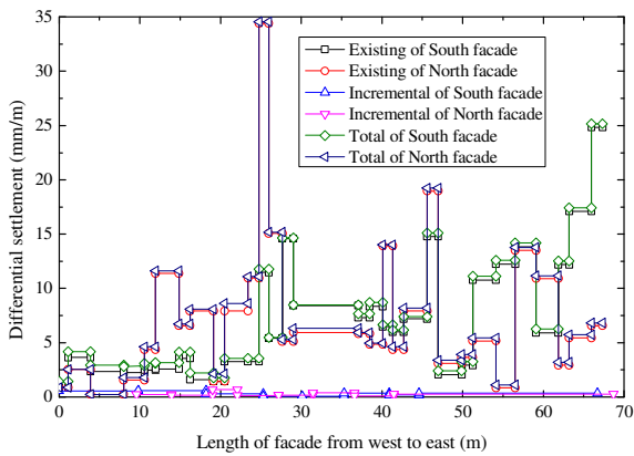
Figure 16 Comparison of existing, incremental and total differential settlements of Chongsi Building
