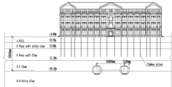
(b) Cross-sectional view of the tunnels and Chongsi Building
