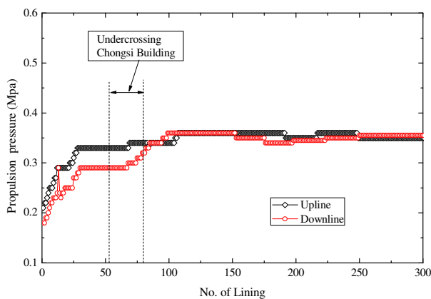
Figure 11 Propulsion pressure of shield tunnels crossing the historic building
