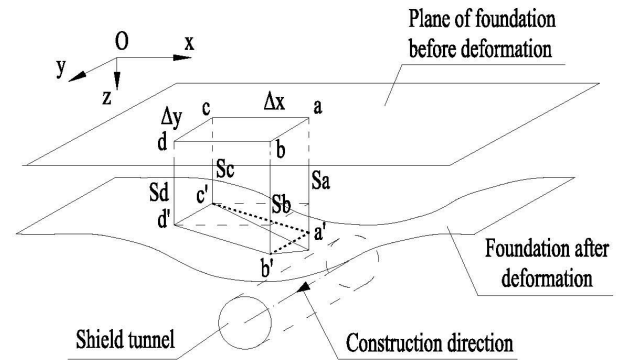
Figure 5 Twist of building foundation
