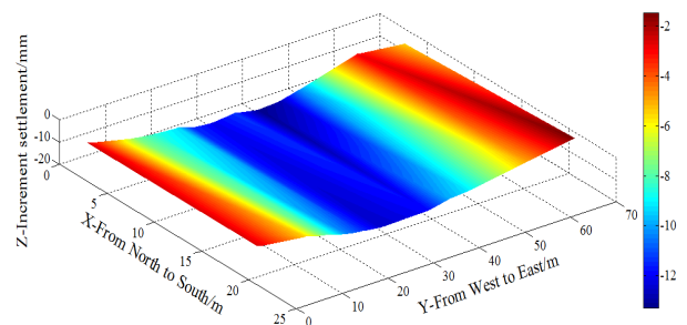
Figure 13 Contours of the settlements
