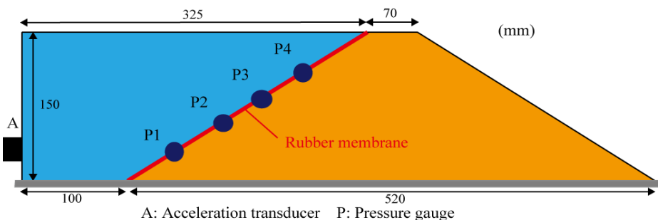
Figure 4 Schematic view of experimental set-up (Model with slope gradient of 1:1.5)
