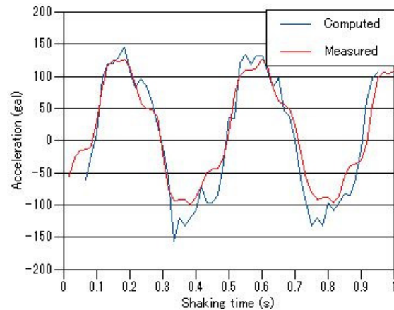
Figure 10 Measured and computed accelerations
