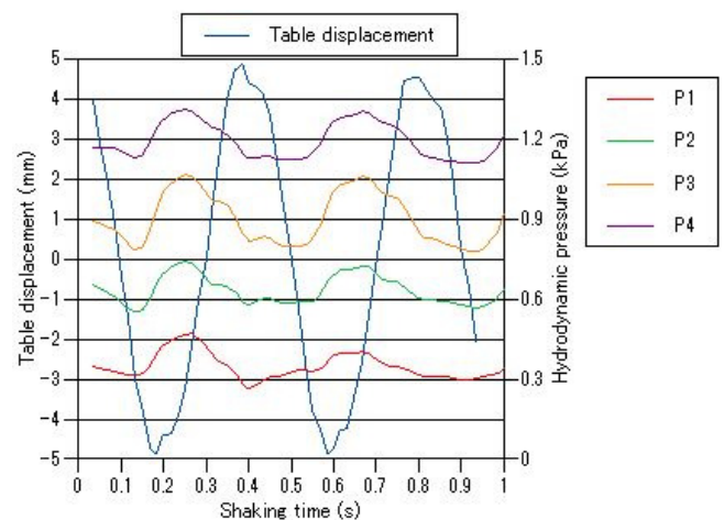
Figure 12 Time histories of displacement of shaking table and hydrodynamic pressure (Large model)
