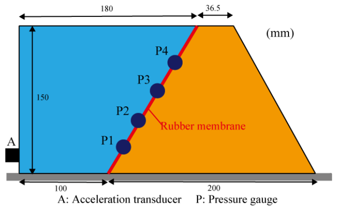
Figure 3 Schematic view of experimental set-up (Model with slope gradient of 1:0.545)
