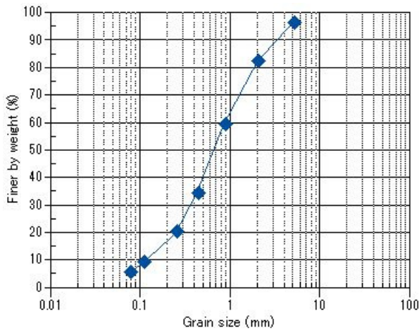
Figure 5 Grain size distribution curve for material
