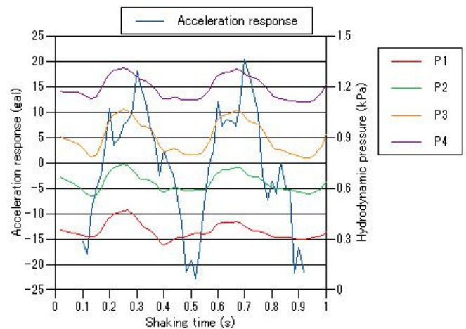
Figure 11 Time histories of acceleration response and hydrodynamic pressure (Large model)
