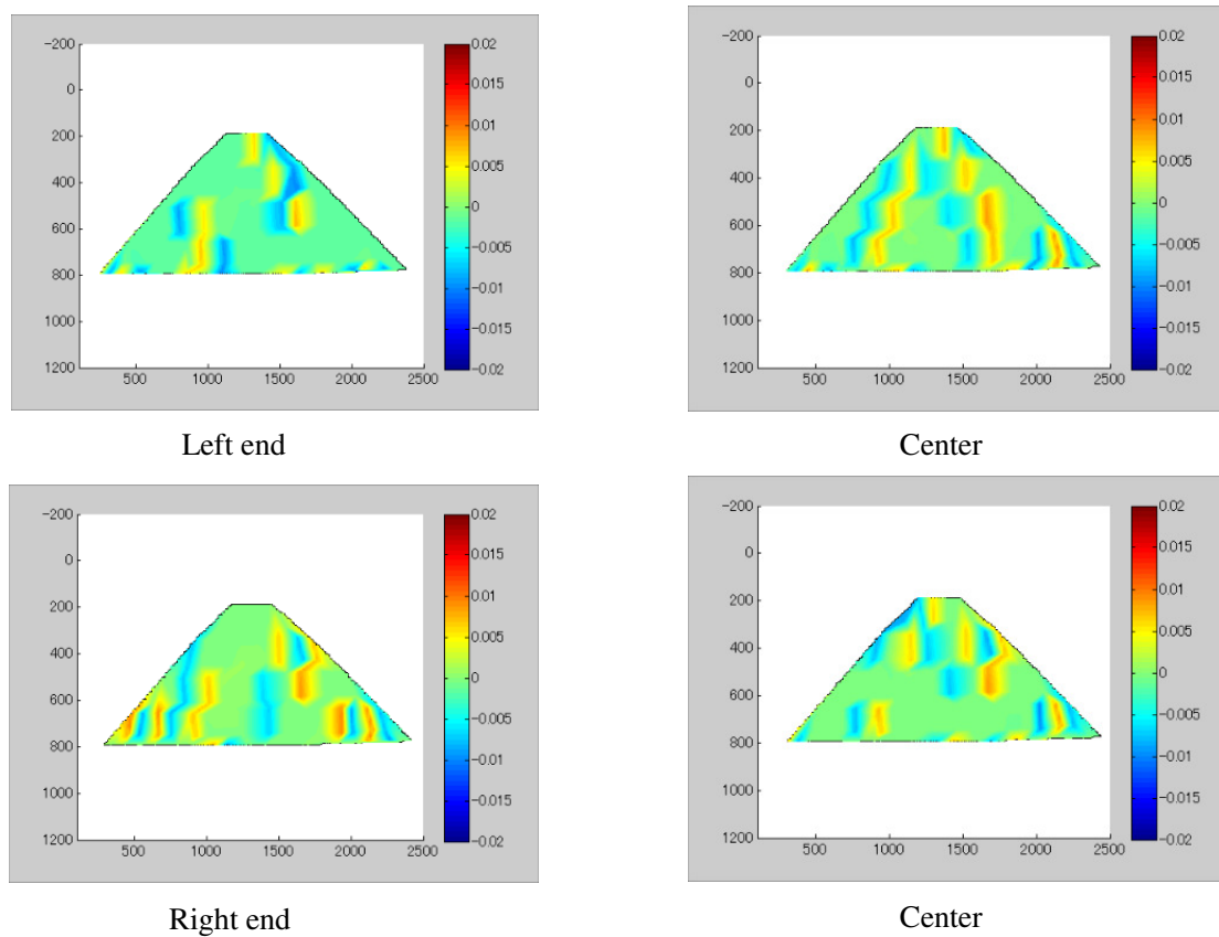
Figure 14 Volumetric strain distributions at left end, center and right end (a) Small model (b) Large model
