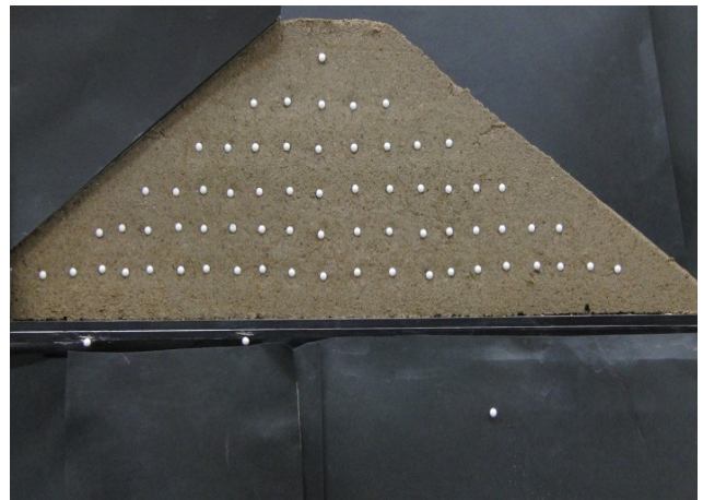
Figure 7 Large model with gauge points
