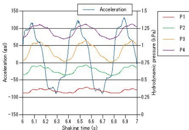
Figure 9 Time histories of measured acceleration and hydrodynamic pressure
