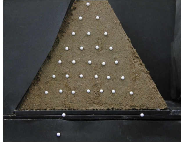
Figure 6 Small model with gauge points
