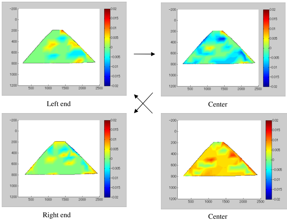
Figure 13 Shear strain distributions at left end, center and right end (a) Small model (b) Large model
