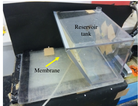
Figure 2 Special water tank with rubber membrane
