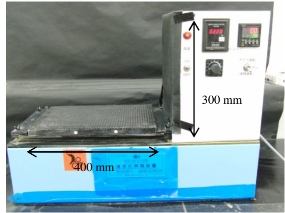
Figure 1 Shaking table
