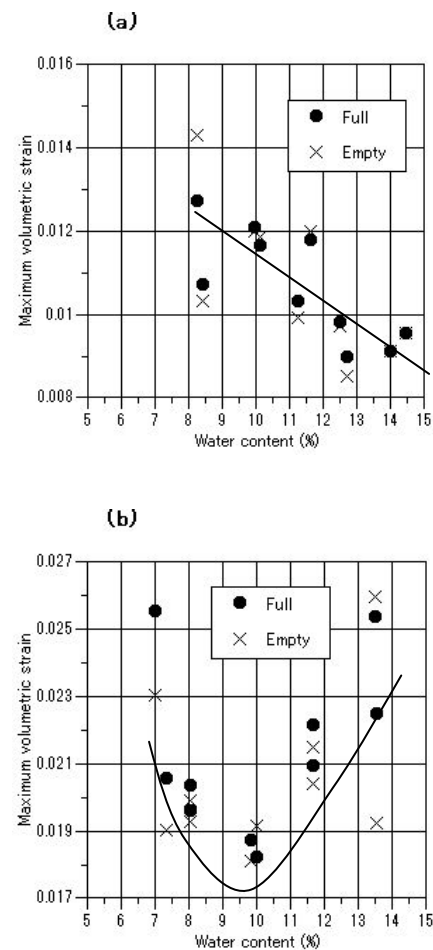
Figure 16 Relationship between maximum volumetric strain and value of water content for (a) Small model and (b) Large model
