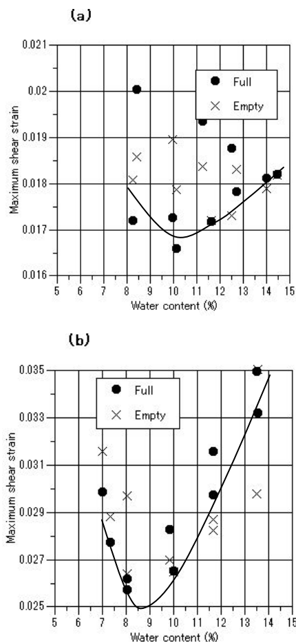
Figure 15 Relationship between maximum shear strain and value of water content for (a) Small model and (b) Large model
