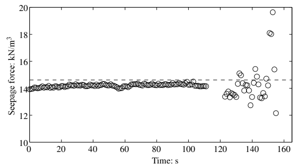
Figure 6 Relationship between seepage force and elapsed time
