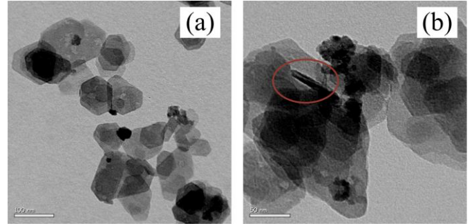
Figure 4 TEM micrographs of loess; (a) original magnification \times 9,700 , and (b) original magnification \times 197,000
