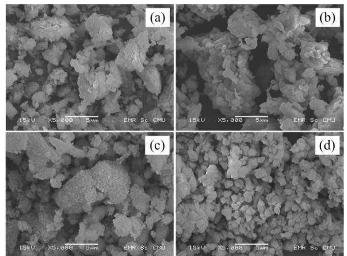
Figure 6 SEM photographs of marble dust waste; (a) raw marble dust waste, (b) marble dust waste calcined at 600 ^{\circ}\text{C} for 2 h, (c) marble dust waste calcined at 800 ^{\circ}\text{C} for 2 h, and (d) marble dust waste calcined at 1,000 ^{\circ}\text{C} for 2 h.
