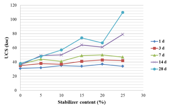
Figure 12 Relationship between UCS and stabilizer content with various curing time
