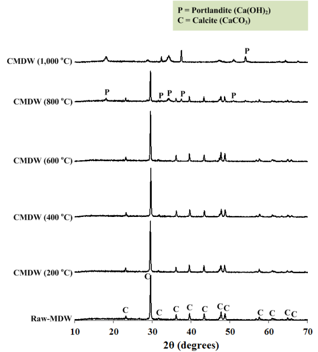
Figure 8 XRD patterns of marble dust waste (Raw-MDW) and marble dust waste calcined at various temperatures
