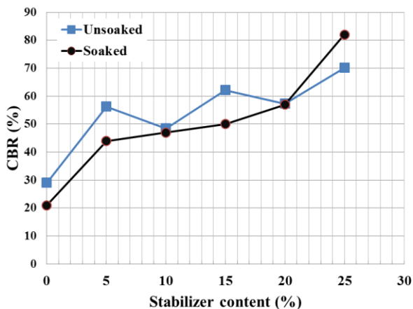
Figure 11 Effect of stabilizer addition on CBR
