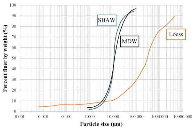
Figure 3 Particle size distribution curves of loess, MDW, and SBAW
