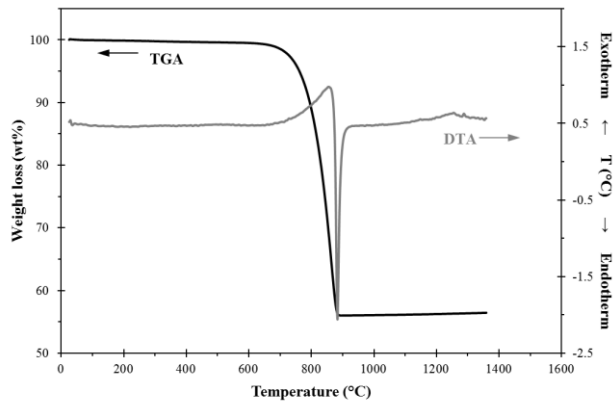
Figure 7 TGA-DTA curves of MDW
