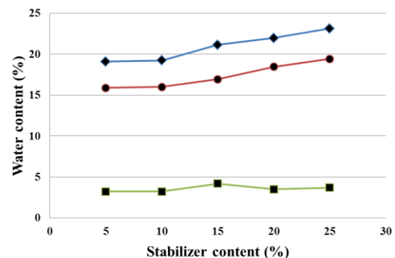
Figure 9 Variation of consistency limits with stabilizer percentage
