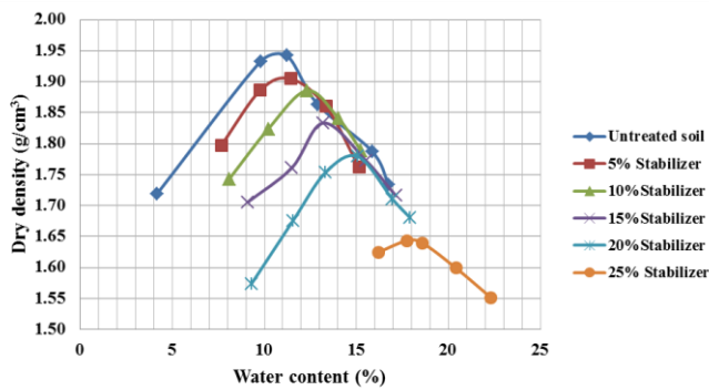
Figure 10 Compaction test results due to the addition of stabilizer to the soil
