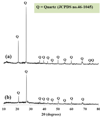
Figure 2 XRD patterns of materials; (a) loess, and (b) SBAW
