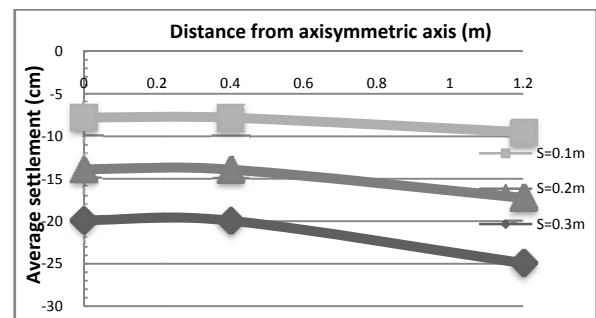
Figure 13 The settlement of the reinforced soft soil surface ( D = 0.8 m; d = 2.4 m)
