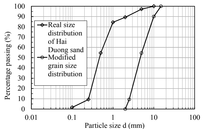
Figure 1 Grain size distribution of Hai Duong sand and modified curve for numerical simulation of triaxial test
