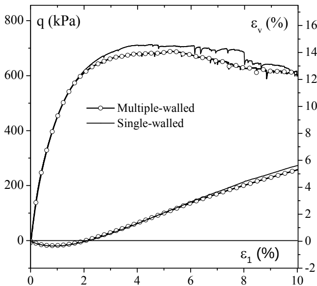
Figure 5 Macroscopic deviatoric stress q and volumetric strain versus axial strain of numerical triaxial tests comparing one-wall and multi-wall boundaries (no rolling, \mu = 0.25 , G_c = 10^9 MPa, \nu_c = 0.25 , \sigma_3 = 200 kPa)
