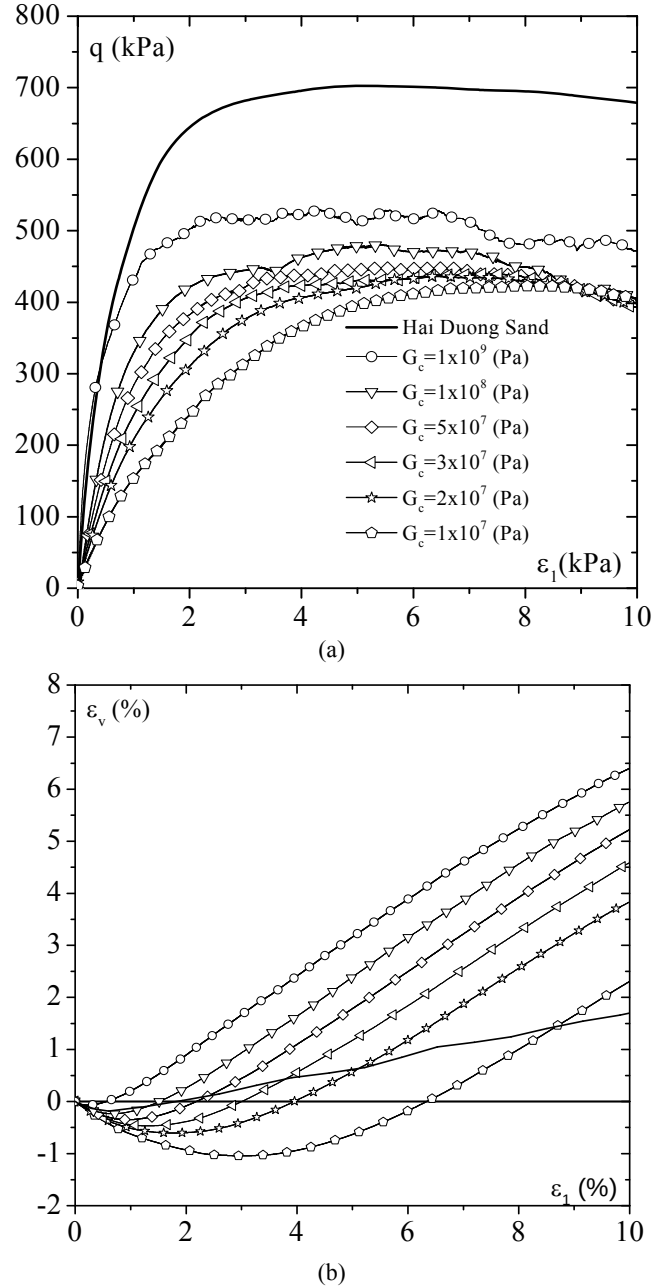
Figure 6 Macroscopic deviatoric stress (a) and volumetric strain (b) versus axial strain of numerical triaxial tests with different contact shear moduli G_c ( \mu = 0.3 , \nu_c = 0.25 , \sigma_3 = 200 kPa)
