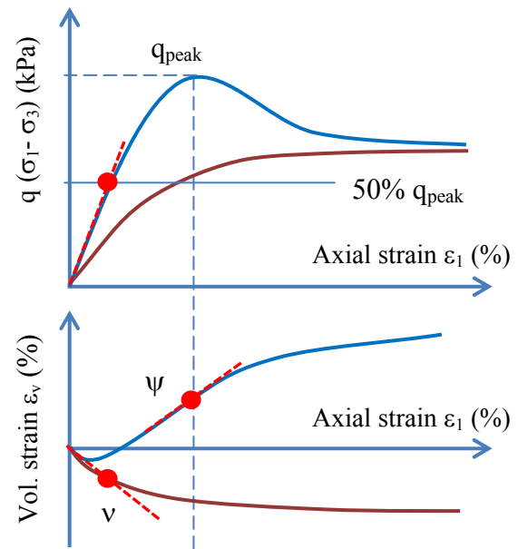
Figure 4 Typical behaviour and corresponding macroscopic parameters of sand under triaxial compression
