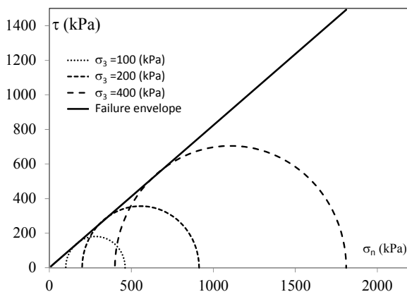
Figure 13 Failure envelope deduced from numerical simulations on Hai Duong sand
