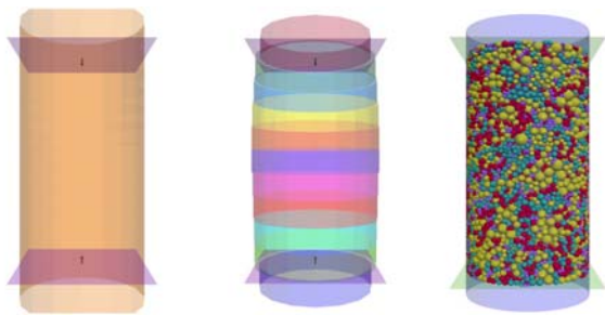
Figure 3 Geometry of models: (a) single-wall boundary; (b) multi-wall boundary (after test); (c) specimen filled with spheres
