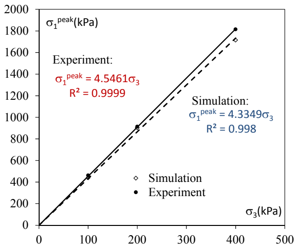
Figure 12 Principal stresses at failure obtained from laboratory experiments and numerical simulations for different confining stresses
