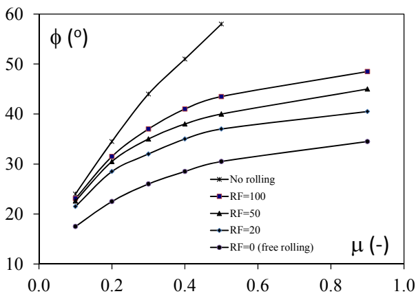
Figure 10 Relation between macroscopic friction angle \phi and microscopic friction coefficient of particles with different values of rolling resistance factor RF ( G_c = 500 MPa, \nu_c = 0.25 , \sigma_3 = 200 kPa)
