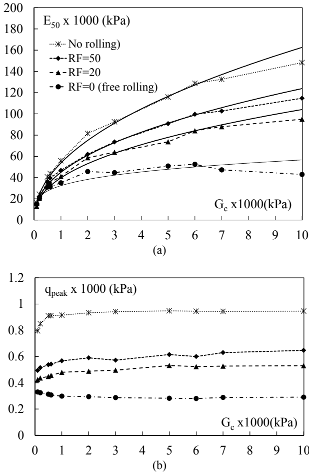
Figure 7 Relationship between (a) macroscopic secant stiffness modulus E_{50} with fitted power functions and (b) macroscopic deviatoric stress q_{peak} versus micro contact shear modulus G_c for different values of rolling resistance factor RF at a confining pressure of 200 kPa.
