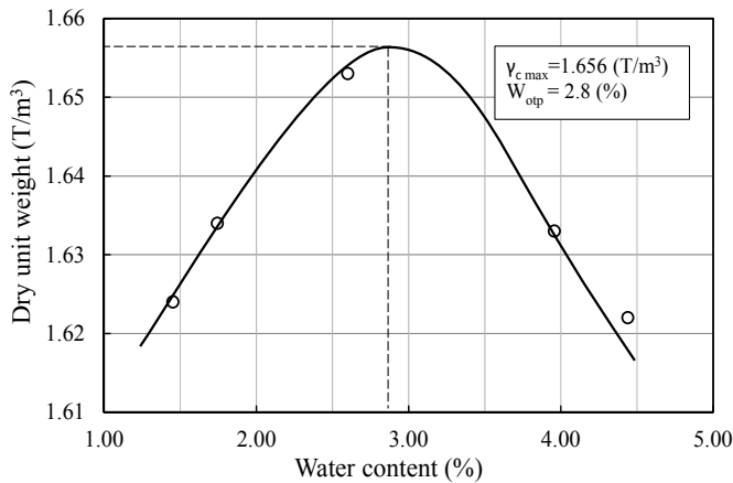
Figure 2 Compaction curve for Hai Duong sand
