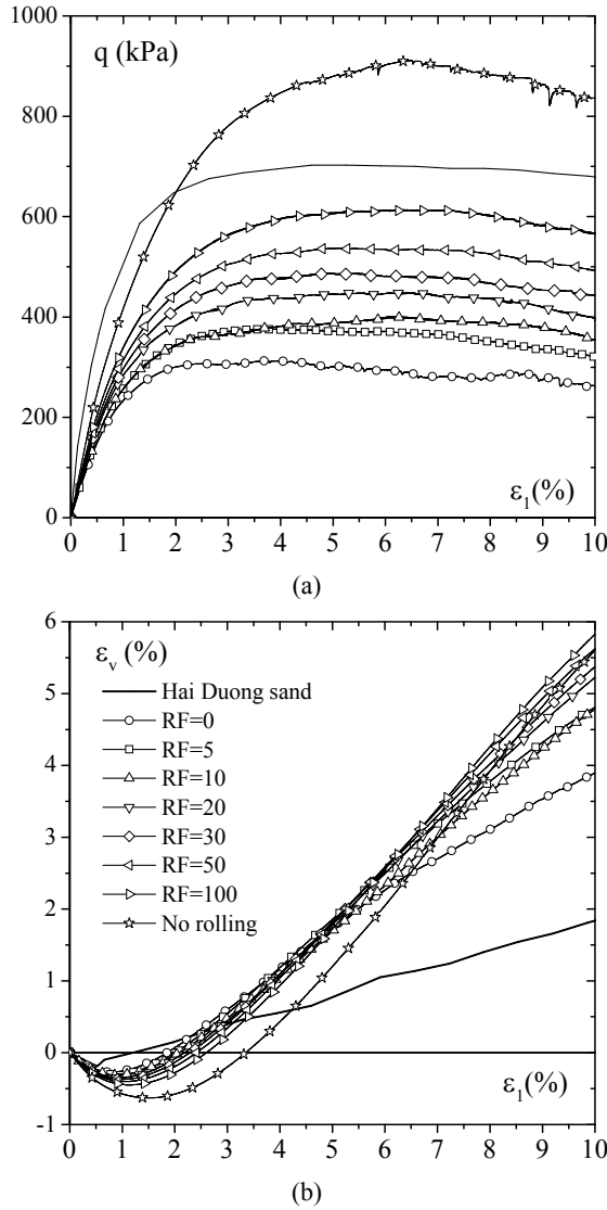
Figure 9 Macroscopic deviatoric stress versus axial strain (a) and volumetric strain versus axial strain (b) of numerical triaxial tests with different rolling resistance factors RF ( \mu = 0.3 , G_c = 500 MPa, \nu_c = 0.25 , \sigma_3 = 200 kPa)
