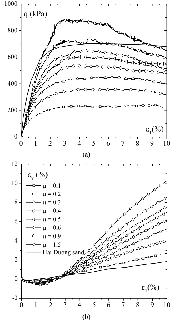
Figure 8 Macroscopic deviatoric stress (a) and volumetric strain (b) versus axial strain of numerical triaxial tests for different contact friction coefficients \mu ( G_c = 500 MPa, \nu_c = 0.25 , \sigma_3 = 200 kPa, RF=20)
