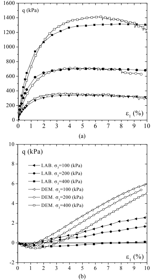
Figure 11 Deviatoric stress and volumetric strain versus axial strain for the laboratory triaxial tests of Hai Duong sand and numerical simulations
