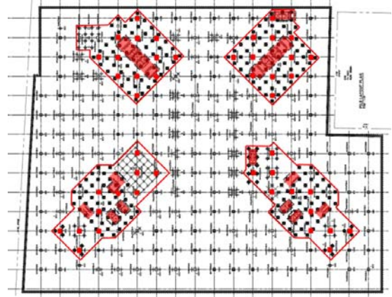
Figure 3 Conventional pile foundation layout
