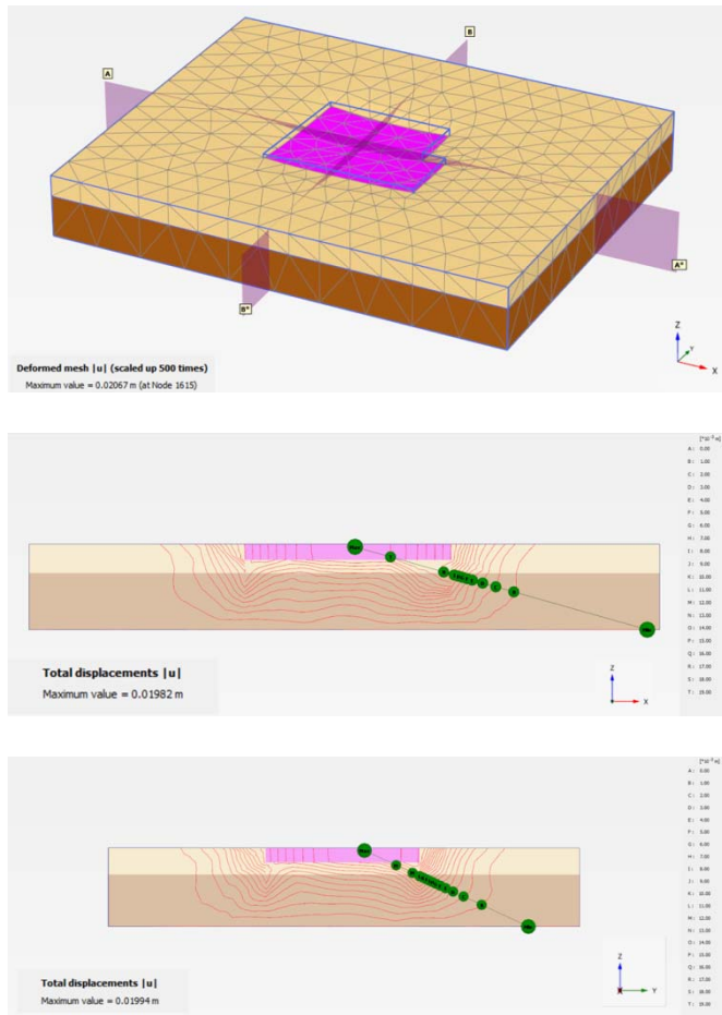
Figure 9 Settlement at cross section along x-x axis (top) and along y-y axis (bottom)
