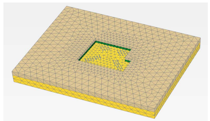
Figure 7 Top view of Plaxis 3D model
