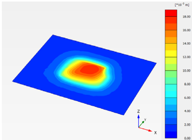
Figure 8 Piled raft-settlement at soil surface level
