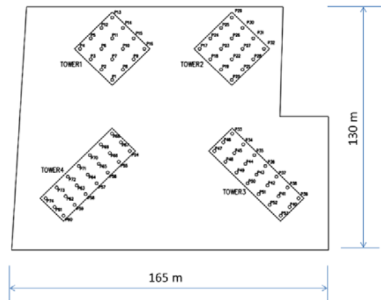
Figure 5 Piled raft foundation - Pile layout
