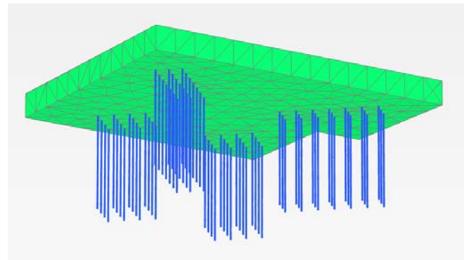
Figure 6 Plaxis 3D piled raft foundation model
