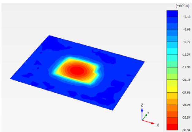
Figure 4 Settlement of the unpiled raft at q_0 = 300 \text{ kPa}
