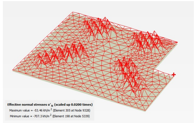
Figure 10 Effective normal stress distributions under the raft bottom
